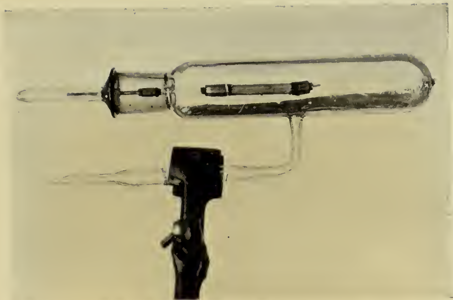
FIG. 16. Professor Strutt's "Radium Clock."
