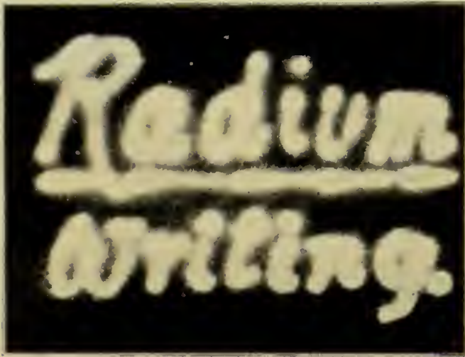
FIG. 6. Written by Radium in the Dark.
