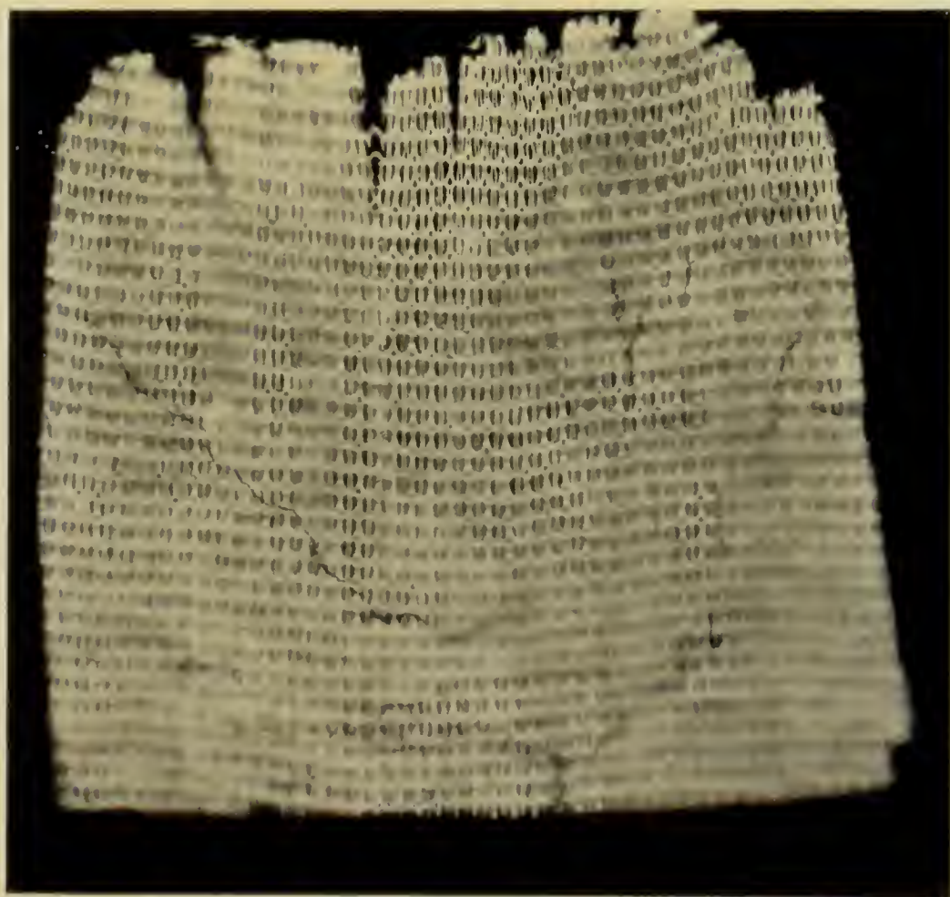
FIG. 2. Welsbach Mantle imprinted by its own rays.
