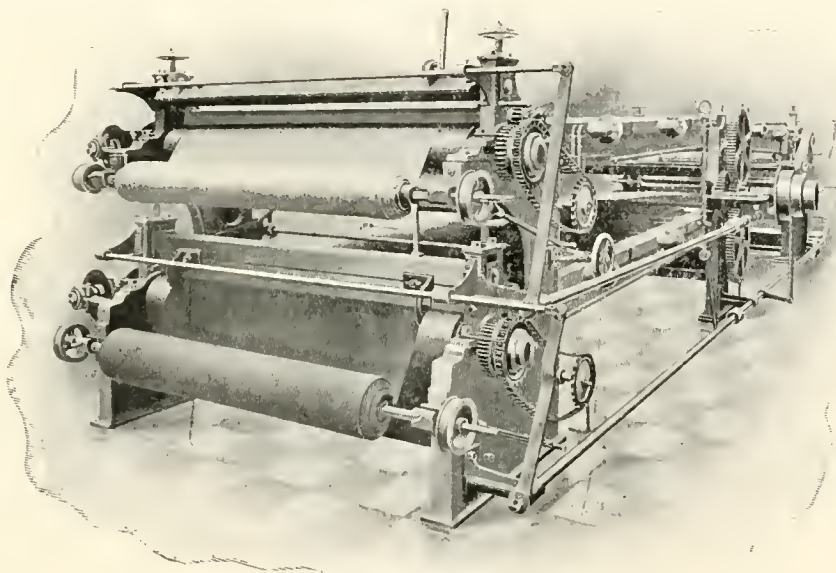
ROWLEY AND WALMSLEY SPREADING MACHINE.
