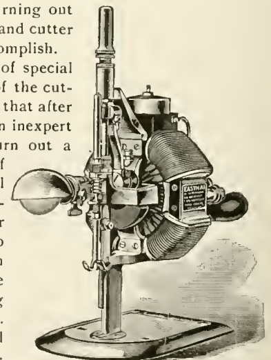
EASTMAN CLOTH CUTTING MACHINE.
