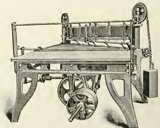
SMITH'S BIAS CUTTING MACHINE.
