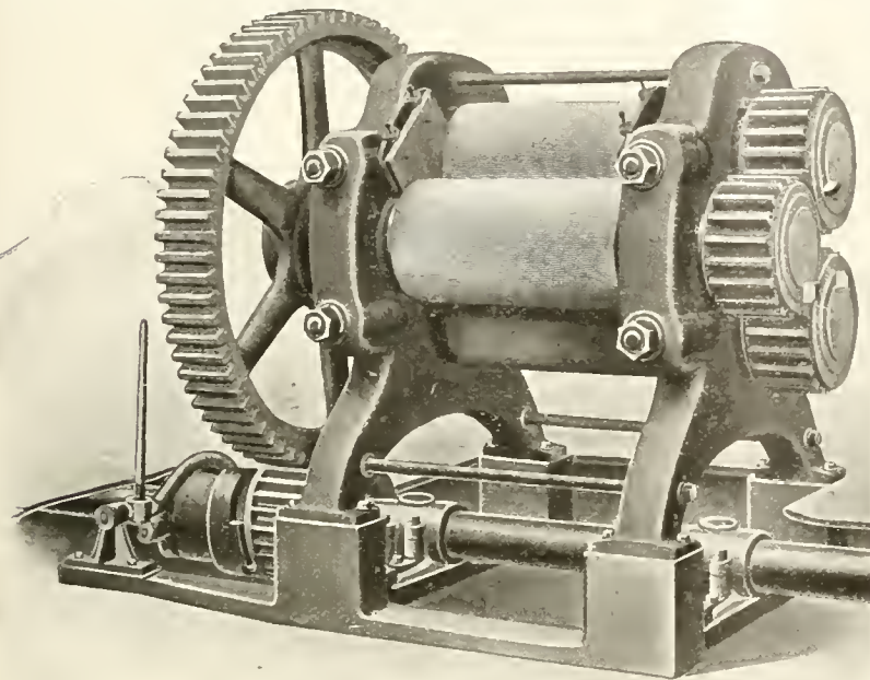
AN AMERICAN THREE ROLL WASHER.
