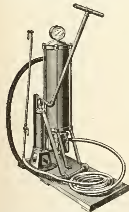
HOOKE'S "BEST" PNEUMATIC COATING MACHINE. F. E. Hook, Hudson, Michigan.
