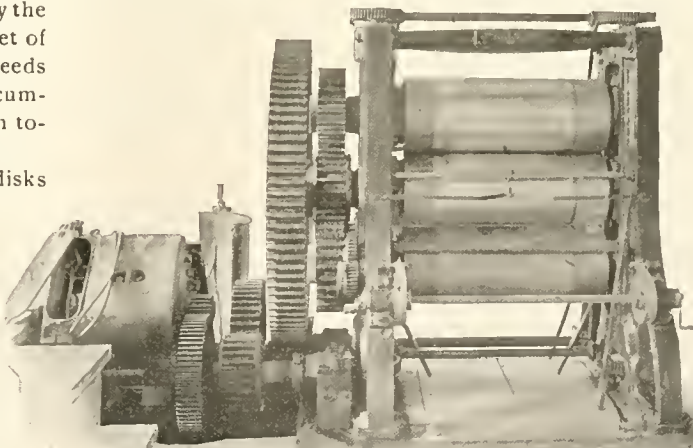
FIG. 3.—CALENDER DRIVEN BY ELECTRIC MOTOR.
