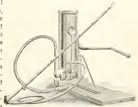
BEAN PNEUMATIC COATING MACHINE. Showing suction hose with strainer; discharge hose; and bamboo rod for ceiling work.—The Bean-Chamberlain Manufacturing Co., Hudson, Michigan.
