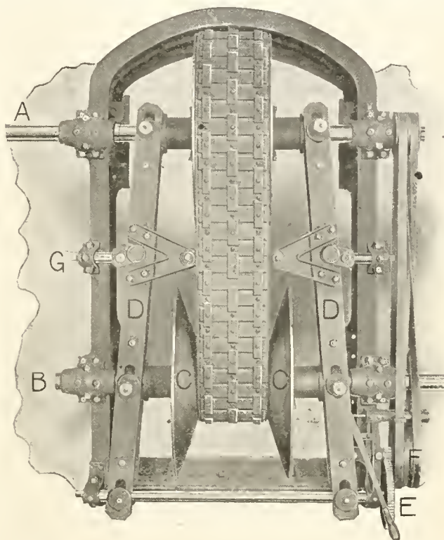
FIG. 2.—REEVES VARIABLE SPEED TRANSMISSION.
