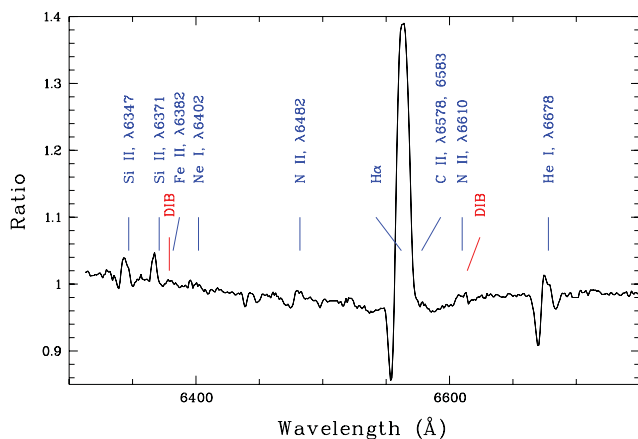
Figure 7. The ratio of the normalized (red) spectra of WS2 obtained within \approx 3 months from each other. The positions of principal lines and most prominent DIBs are indicated.
