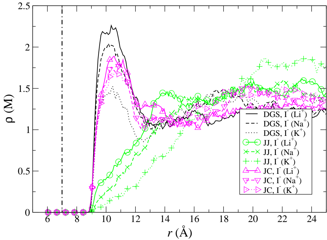
FIG. 8: Iodide radial density profiles around a cylindrical solute of \varepsilon_{in} = 2 for cation-iodide salts with different cation counterparts for the three ion models.
