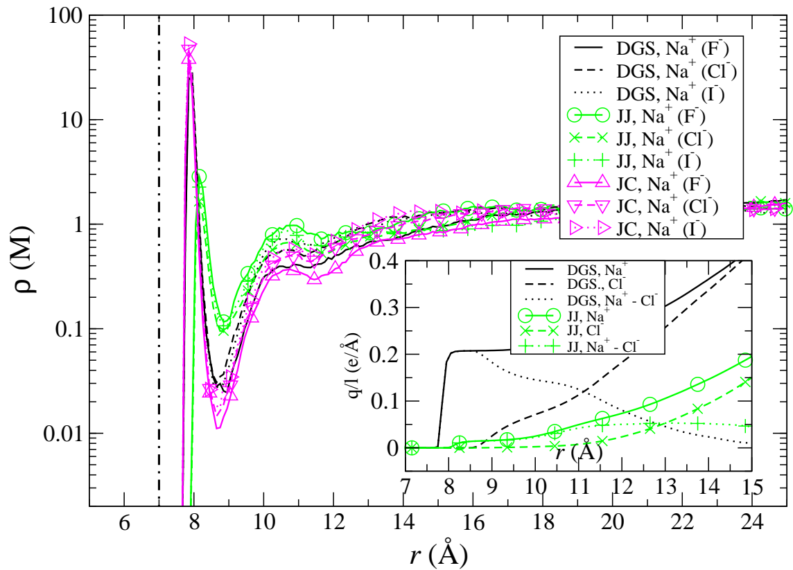
FIG. 9: Sodium radial density profiles around a cylindrical solute of \epsilon_{in} = 5 for sodium-anion salts with different anion counterparts for the three ion models. (Inset) Cumulative (integrated) Na + and Cl - radial ion densities and their difference showing the dependence on the ion models.
