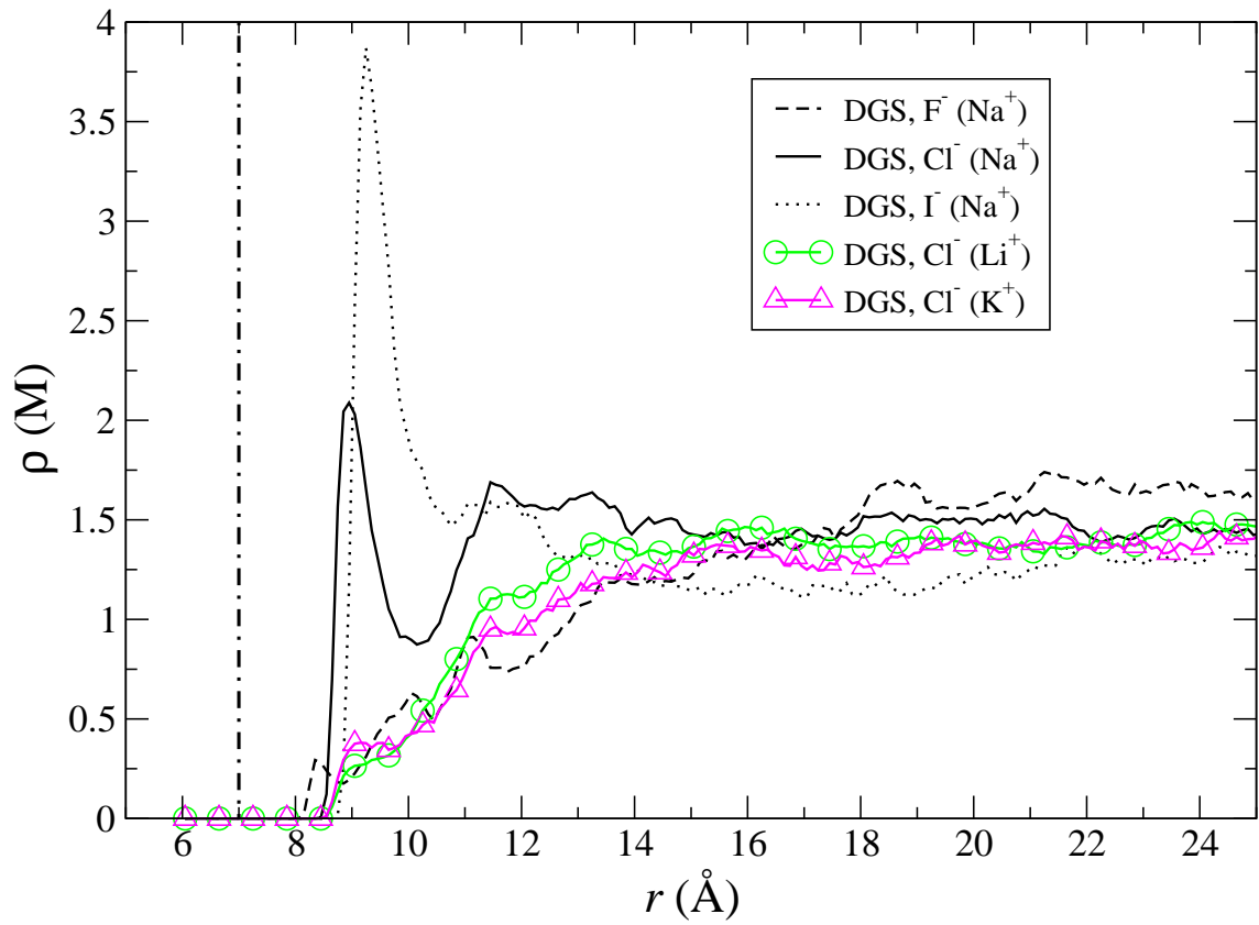
FIG. 14: Radial density profiles of anions around a cylindrical solute of \varepsilon_{in} = 5 for various salts.
