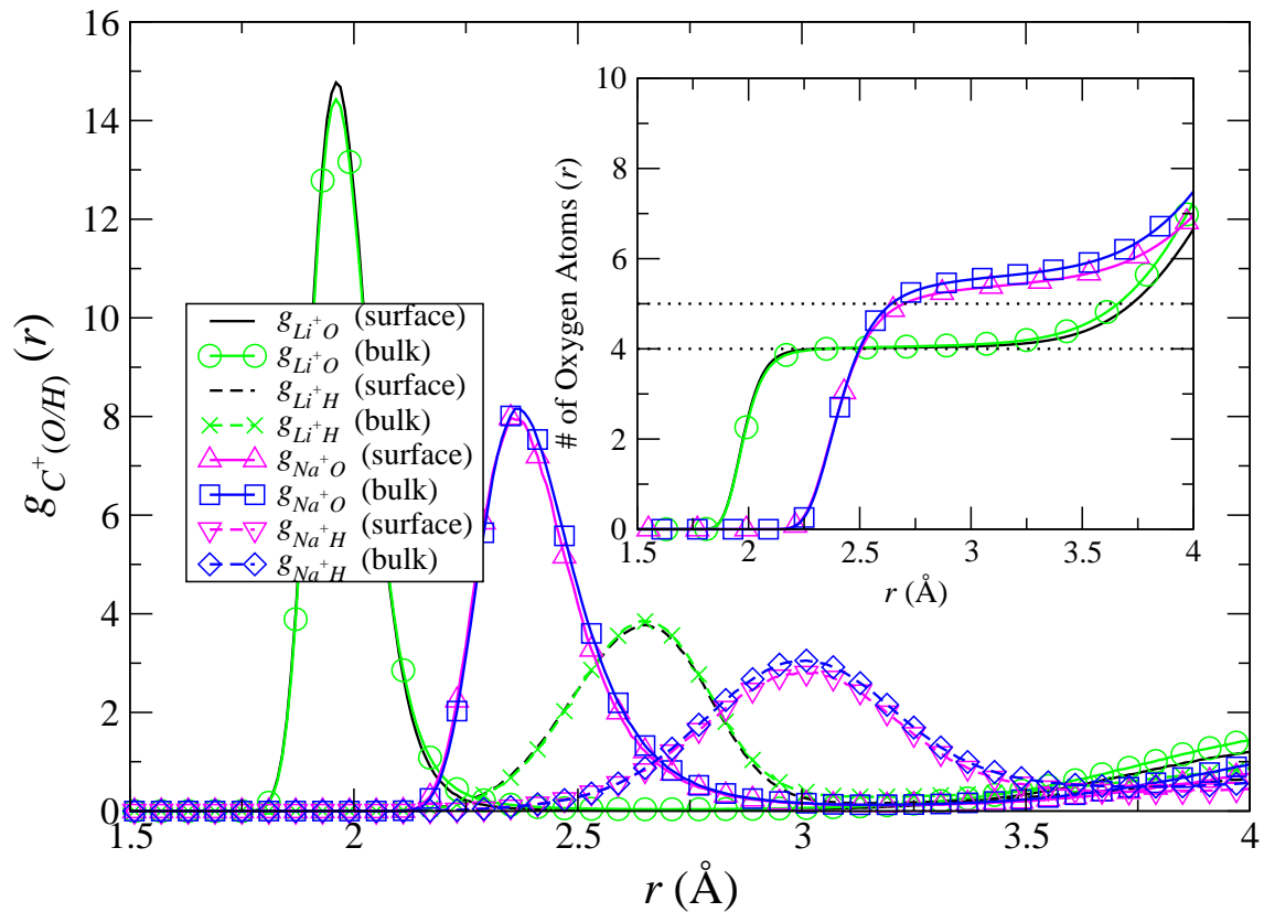
FIG. 5: The radial distribution functions of water about the Li^+ and Na^+ ions in (DGS) LiCl and NaCl salt simulations of a cylindrical solute of \epsilon_{in} = 2 . Curves labeled “surface” correspond to the rdf’s of ions within \approx 3\text{\AA} of the solute surface, which accounts for those ions within the peak ( r < 11\text{\AA} ) of the Li^+ distribution shown in Fig. 4. Note the slightly larger Li^+ -O peak for ions near the surface. (Inset) The integrated rdf, which reveals the coordination number of water molecules in the ions’ first solvation shells.
