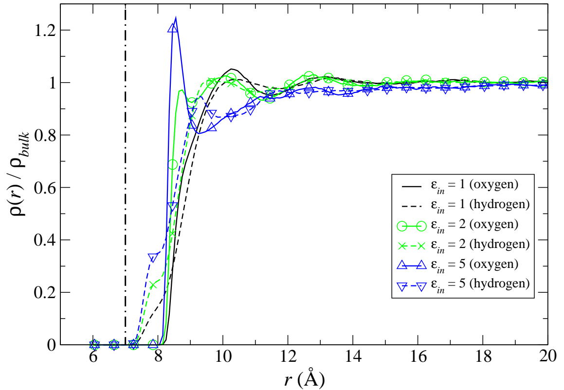
FIG. 1: Oxygen and hydrogen radial density profiles around the cylindrical solute as a function of solute permittivity. The vertical dash-dot line in this plot, and all following plots, shows the location of the cylindrical solute hard wall, which is also the location of the image charge plane ( R_c = 7\text{\AA} ).
