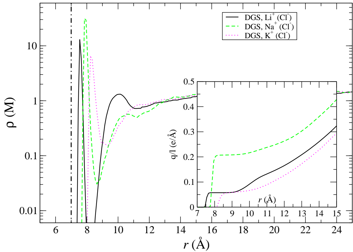
FIG. 10: Radial density profiles of the cations around a cylindrical solute of \varepsilon_{in} = 5 for cation-chloride salts. (Inset) The corresponding cumulative (integrated) radial ion densities.
