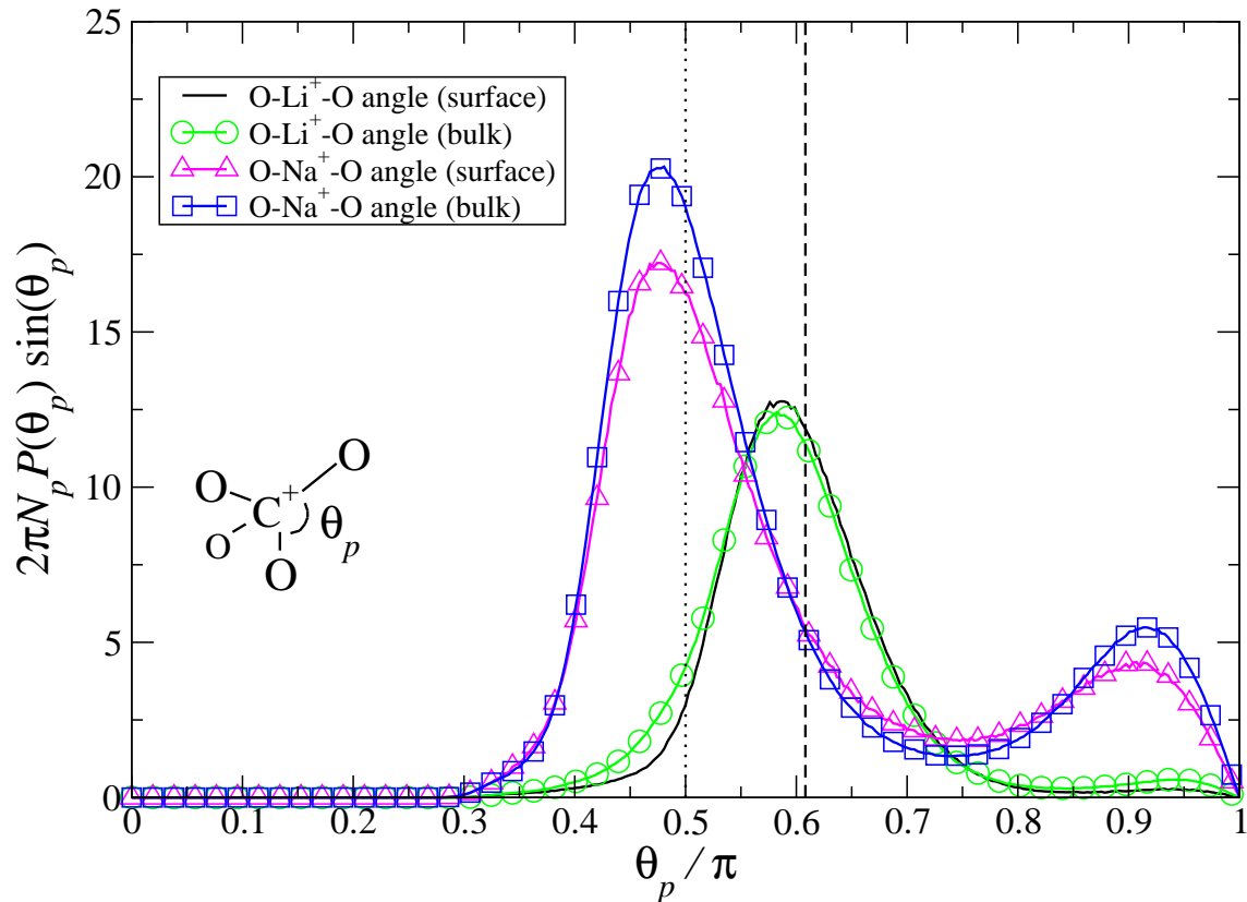
FIG. 6: The probability distribution, such that \int P(\theta_p) d\Omega = 1 for each of the O-C + -O “bond” pair angles, of the “bond” angle defined by the two vectors connecting the cation and two of the water oxygen atoms in the first solvation shell for (DGS) LiCl and NaCl salt simulations. The dashed line corresponds to the tetrahedral angle ( \arccos(-1/3) = 109.5^\circ ) and the dotted line to the octahedral angle ( 90^\circ ). N_p corresponds to the number of distinct O-C + -O configurations of the water oxygen atoms within the first solvation shell, e.g., for four-fold water coordination about the cation, N_p = 6 .
