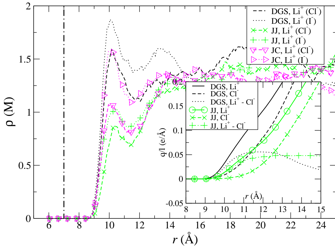
FIG. 4: Lithium radial density profiles around a cylindrical solute of \varepsilon_{in} = 2 for lithium-anion salts with different anion counterparts for the three ion models. (Inset) Cumulative (integrated) \text{Li}^+ and \text{Cl}^- radial ion densities and their difference showing the dependence on the ion models.
