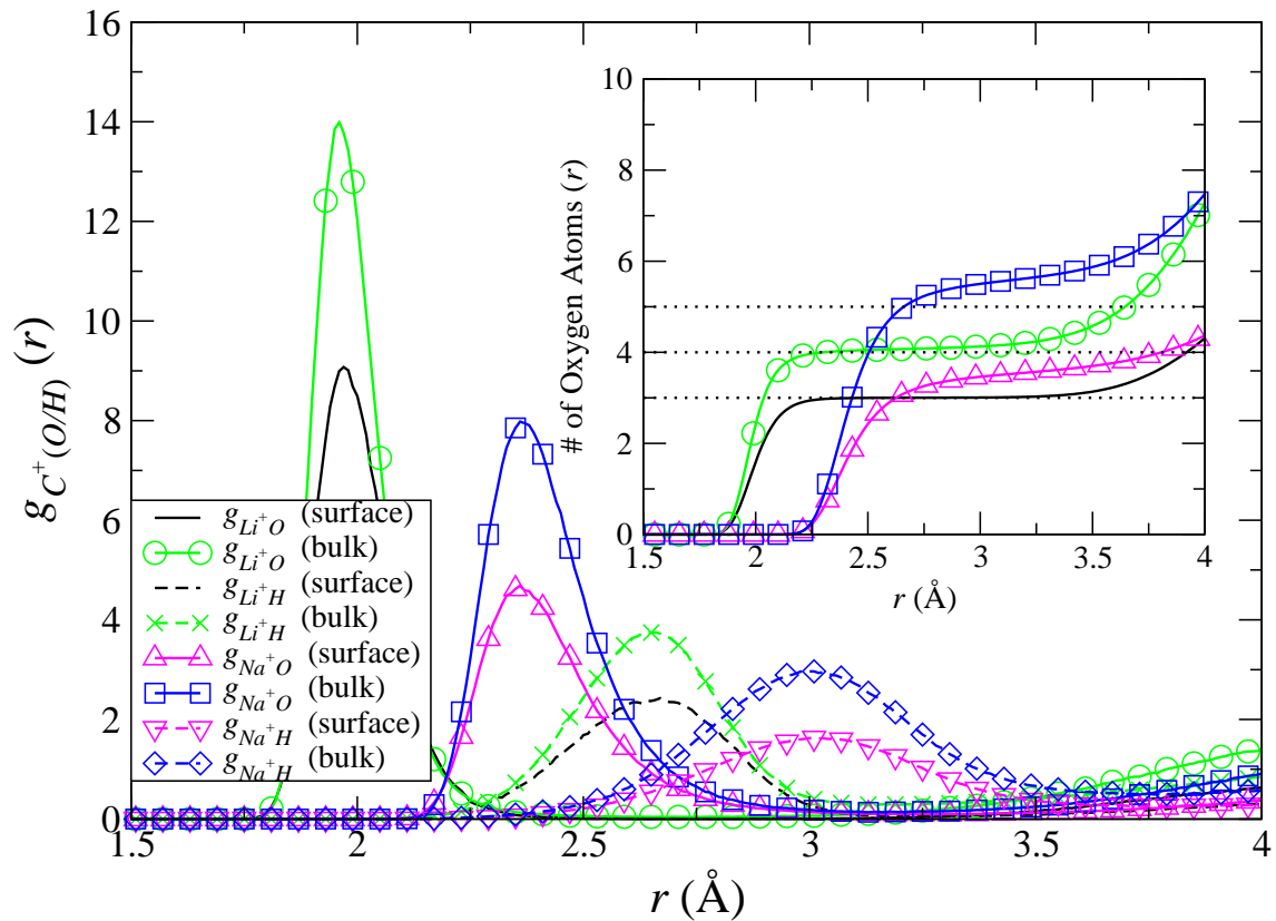
FIG. 11: The radial distribution functions of water about the Li^+ and Na^+ ions in (DGS) LiCl and NaCl salt simulations of a cylindrical solute of \epsilon_{in} = 5 . Curves labeled “surface” correspond to the rdf’s of ions within \approx 1\text{\AA} of the solute surface, which accounts for those adsorbed ions within the peak ( r < 9\text{\AA} ) of the cation distribution shown in Fig. 10. (Inset) The integrated rdf, which reveals the reduction of the coordination number of water molecules in the ions’ first solvation shells for ions near the solute surface as compared to bulk. Here, the Li^+ coordination number is reduced by one water molecule, whereas that for Na^+ is reduced by two.
