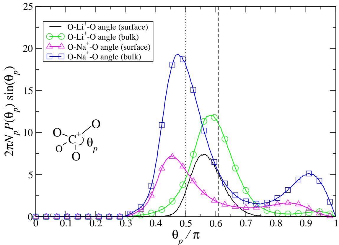
FIG. 12: The probability distribution of the “bond” angle defined by the vectors connecting the cation and two of the water oxygen atoms in the first solvation shell for (DGS) LiCl and NaCl salt simulations. The dashed line corresponds to the tetrahedral angle ( \arccos(-1/3) = 109.5^\circ ) and the dotted line to the octahedral angle ( 90^\circ ). The bonding configurations for both adsorbed Li + and Na + remain relatively unchanged as compared to the \epsilon_{in} = 2 case, with Li + having a tetrahedral-like arrangement within its solvation shell and Na + having a slightly distorted octahedral arrangement. (See Fig. 13.)
