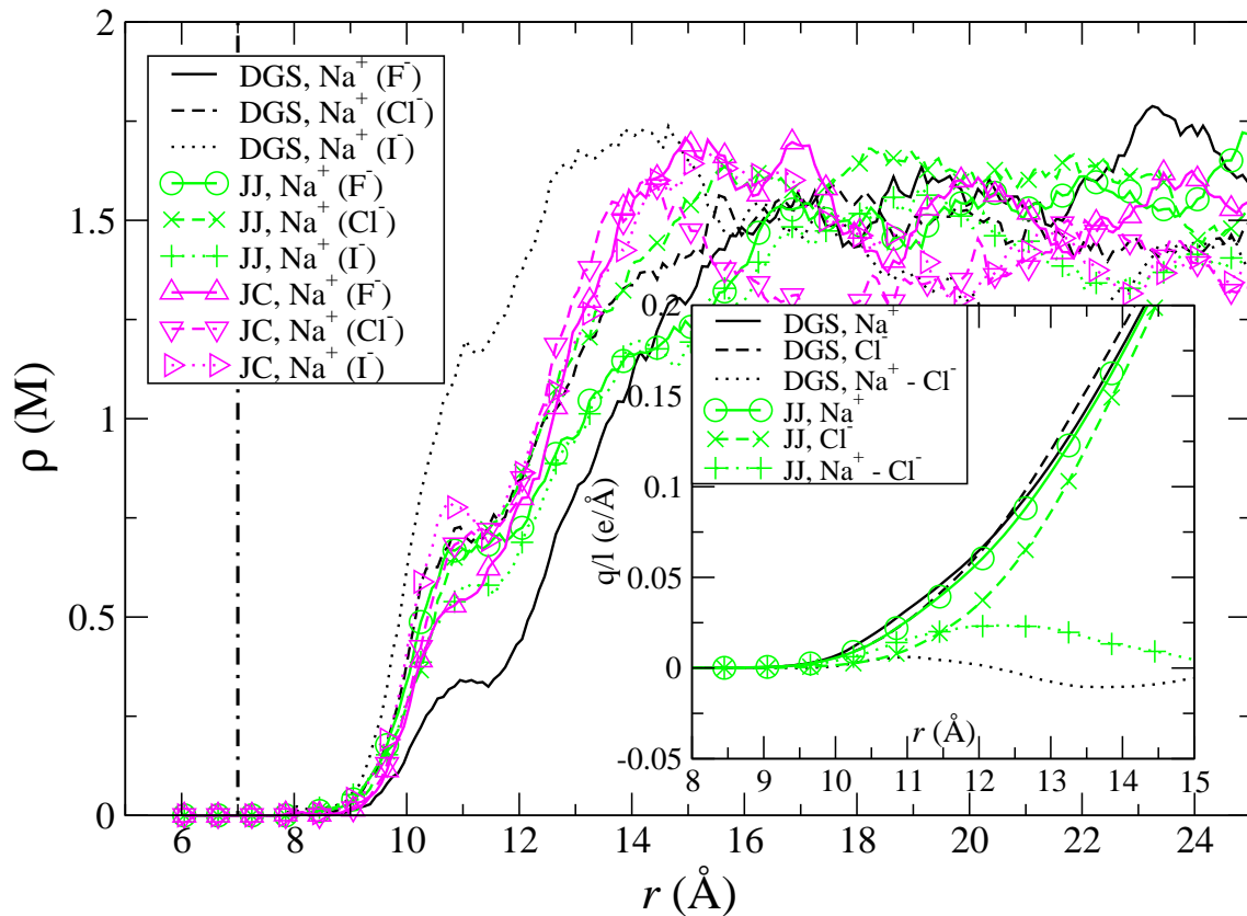
FIG. 3: Sodium radial density profiles around a cylindrical solute of \epsilon_{in} = 2 for sodium-anion salts with different anion counterparts for the three ion models. (Inset) Cumulative (integrated) \text{Na}^+ and \text{Cl}^- radial ion density and their difference showing the dependence on the ion models. (Note that the salt ion concentrations in this and subsequent figures are defined in terms of molarity, rather than molality, so that the number of ions in a given volume can be easily worked out in these systems. Again, the bulk water density is found to change when varying salt species.)
