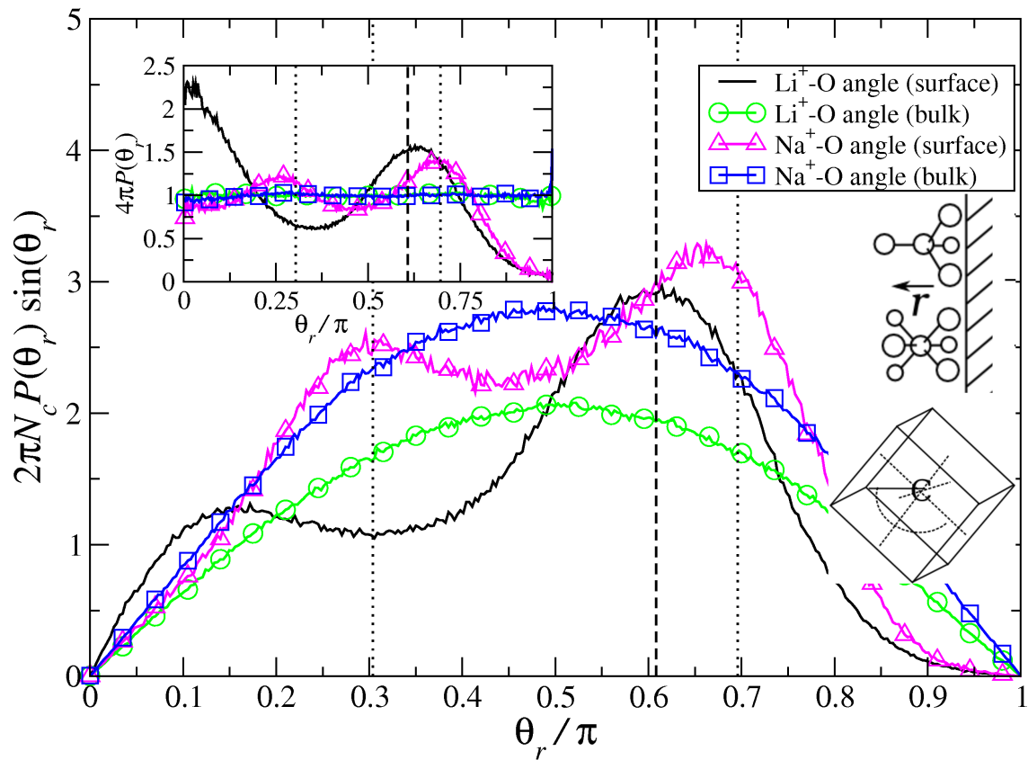
FIG. 7: The normalized probability distribution, without the solid angle correction, of the angle between the vector connecting the cation and a water oxygen atom in the first solvation shell and the radial vector from the solute axis to the cation location for (DGS) LiCl and NaCl salt simulations. The dashed line corresponds to the tetrahedral angle ( \arccos(-1/3) = 109.5^\circ ) and the dotted lines to the angle ( \arccos(\pm(1/\sqrt{3})) ) between the face-centered bond vectors and the corner (or opposite corner) of a cube defined by the octahedral bonding structure as diagrammed in the figure. N_c corresponds to the coordination number of water molecules about the cation. (Inset) The solid-angle corrected distribution which takes into account the polar-angle weighting.
