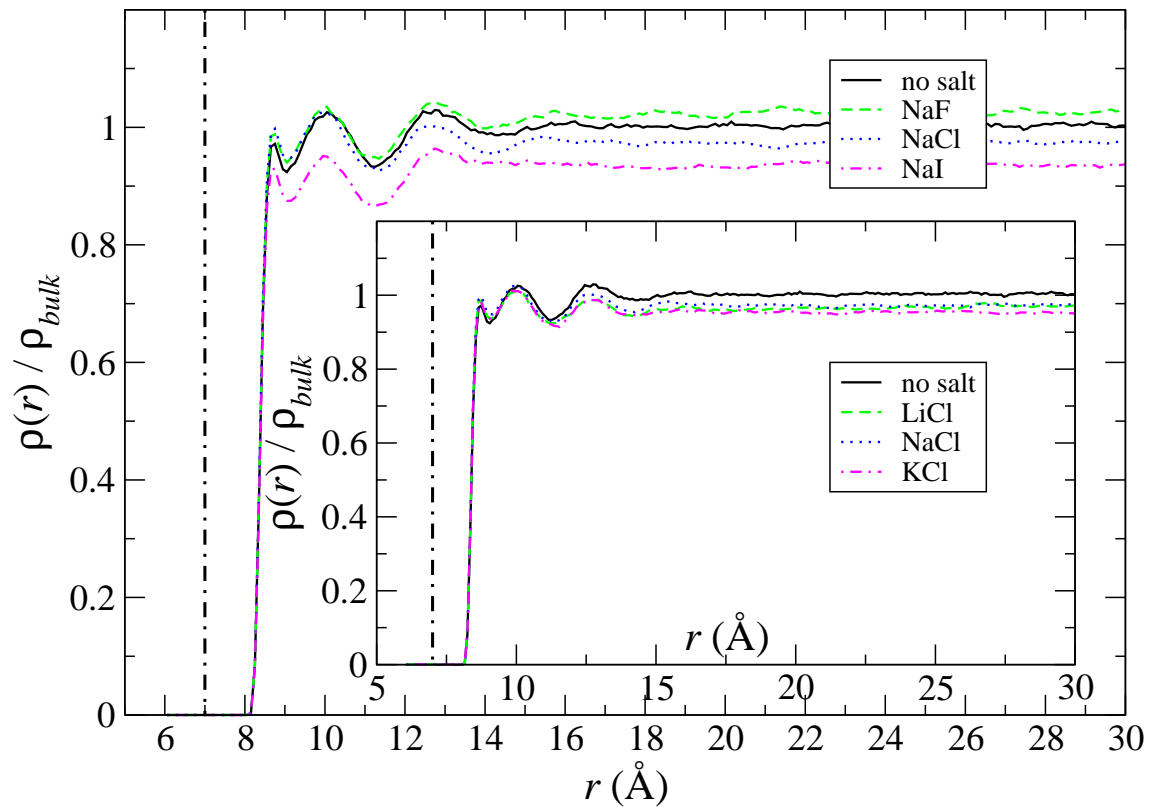
FIG. 2: Oxygen radial density profiles around a cylindrical solute of \epsilon_{in} = 2 for sodium-anion salts with different anion counterparts (Inset: cation-chloride salts with different cations) for the DGS ion models.
