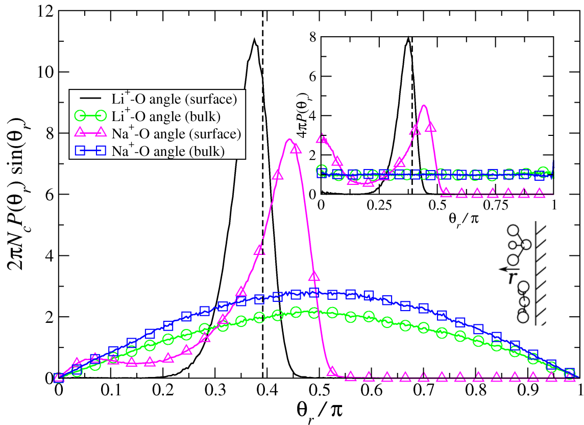
FIG. 13: The probability distribution of the angle between the vector connecting the cation and a water oxygen atom in the first solvation shell and the radial vector from the solute axis to the cation location for (DGS) LiCl and NaCl salt, \varepsilon_{in} = 5 simulations. The dashed line corresponds to the supplement of the tetrahedral angle ( 180^\circ - \arccos(-1/3) = 70.5^\circ ). According to these distributions and those shown in the previous figure (Fig. 12), the water bonding structure may be extracted and is given by the diagram within this figure. Here, as opposed to the \varepsilon_{in} = 2 case, the legs of the tetrahedron of the Li + point away from the solute surface, providing a three-fold coordination for Li + . Likewise, the distributions suggest a distorted (away from the surface) square planar structure for the larger Na + ion, with a coordination number between three and four (see Fig. 11). (Inset) The solid-angle corrected distribution which takes into account the polar-angle weighting.
