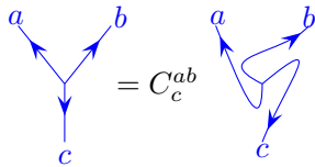
Fig. 14.26 The relationship between these two diagrams is unitary, meaning C is a just a phase. For cases where N_{ab}^c > 1 the vertices are marked with an index, say \mu on the left and \nu on the right, and for fixed a , b , and c , the constant C_c^{ab} becomes a unitary matrix [C_c^{ab}]_{\mu\nu} in the indices \mu, \nu .
