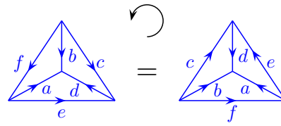
Fig. 16.17 An obvious rotational symmetry of the tetrahedral diagram.
