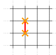
Fig. 25.9 Starting in the code space, a \sigma_x operator applied to the red edge ( i ) creates two vertices in the V_\alpha = -1 eigenstate marked with the orange \times 's.
