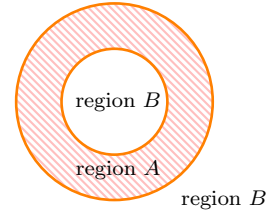
Fig. 33.4 Partitioning a system into two regions. In this case region A is the shaded region and B is the unshaded region (which is split between inside and outside).
