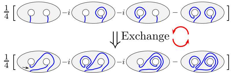
Fig. 30.6 Calculation of the phase accumulated from exchanging two \gamma particles. The upper line represents two \gamma quasiparticles, one in each hole (Compare Eq. 30.7). The holes are exchanged, braiding the blue lines in the process. Using surgery and loop addition/removal (the moves of Eq. 30.1 and 30.2) one can show the lower line is precisely -i times the top line showing an exchange phase of -i . For example, the first term in the second line is equivalent to the second term in the first line times -i .
