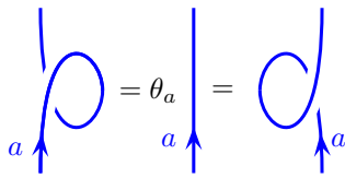
Fig. 15.2 The definition of the twist factor \theta_a drawn using blackboard framed diagrams. The curled strings should be thought of as ribbons lying in the plane as in Fig. 15.1 which are equivalent to a ribbon that twists around its own axis.
