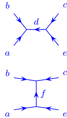
Fig. 20.7 Fusion of representations. Compare to the diagrams in Fig. 16.3. The top figure can be thought of as the d component of \mathcal{R}_a \otimes \mathcal{R}_b \simeq \bigoplus_{\bar{d}} N_{ab}^{\bar{d}} \mathcal{R}_{\bar{d}} fused with \mathcal{R}_c \otimes \mathcal{R}_e \simeq \bigoplus_d N_{ce}^d \mathcal{R}_d to form the identity. The bottom figure can be thought of as the f component of \mathcal{R}_b \otimes \mathcal{R}_c \simeq \bigoplus_{\bar{f}} N_{bc}^{\bar{f}} \mathcal{R}_{\bar{f}} fused with \mathcal{R}_a \otimes \mathcal{R}_e \simeq \bigoplus_f N_{ae}^f \mathcal{R}_f to form the identity.
