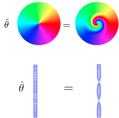
Fig. 28.13 Deforming the environment of a particle (top) implements the twist operation. This is equivalent to the space-time diagram shown on the bottom (See also chapter 15)
