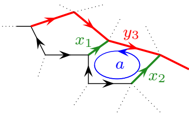
Fig. 29.20 The measurement of x_1x_2x_3 \dots commutes with the application of P_\beta(h) to the shown plaquette, since P_\beta(a) takes x_1 \rightarrow x_1a^{-1} and takes x_2 \rightarrow ax_2 . Note that in this figure we have reversed the orientation of x_3 such that all of the green arrows point in the same direction with respect to the ribbon (bright green in Fig. 29.19).
