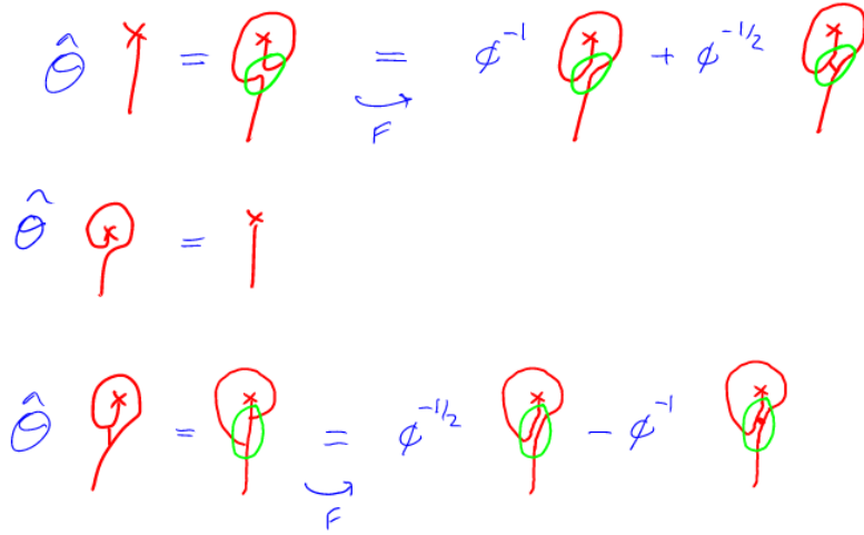
Fig. 31.12 The rotation operator \hat{\Theta} applied to the possible string endings. Then using F matrices we reduce the results to linear combinations of the same endings.
