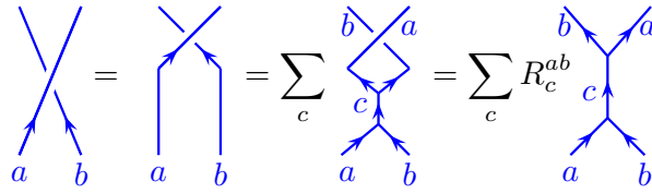
Fig. 13.7 A generic crossing can be reduced to a planar diagram using the R -matrix. In the second step a complete set of particles c is inserted as in Fig. 12.20. Note this figure uses physics normalization.
