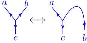
Fig. 14.24 A theory is pivotal if there exist isomorphisms between the states of the Hilbert spaces described by pairs of vertices that differ by downturning and upturning lines.
