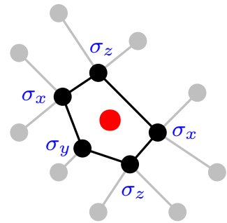
Fig. 32.5 A closeup of one of the dislocations in Fig. 32.4. For the 5-sided plaquette, the 3-valent vertex is assigned \sigma_y whereas the north, east, south, and west vertices are assigned \sigma_z, \sigma_x, \sigma_z, \sigma_x as in all of the four-sided plaquettes.
