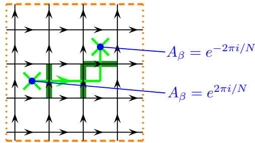
Fig. 25.24 Application of the operator X_j = e^{2\pi i s_j / N} on an edge (shown as dark green lines) multiplies the eigenvalue of A_\beta on the plaquette to the left of the arrow by e^{2\pi i / N} and multiplies the eigenvalue of the plaquette to the right by e^{-2\pi i / N} . Multiple applications of these operators can move the defective plaquettes away from each other, as shown in the Figure — only the bright green \times 's are defects. In the figure, the two vertical dark green bonds are X_j operators and the horizontal dark green bond is a X_j^{-1} operator.
