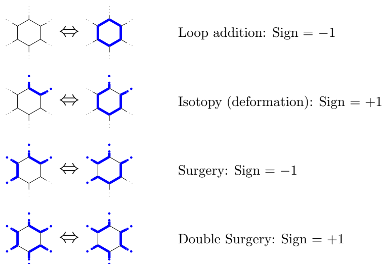
Fig. 30.1 When flipping over a plaquette, the sign is -1 if the number of loops in the system changes parity. A “leg” of the plaquette is one of the edges pointing out of the plaquette, i.e., having only one end on a vertex of the plaquette (these are drawn partially dotted in the figure). Let the number of blue legs of the plaquette be L , which is always even as long as we have no vertex defects. The sign associated with flipping the plaquette is -1 if L/2 is even and is +1 otherwise. This rule holds for plaquettes with any number of sides.
