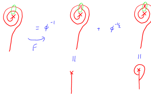
Fig. 31.11 An example of reducing a more complicated string ending into one of the three endings shown in Fig. 31.10.
