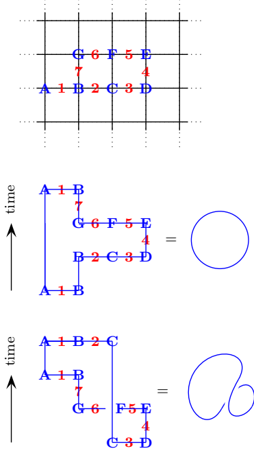
Fig. 26.2 Top: Vertices are labeled with letters and edges with numbers. Middle: The process shown is (reading right to left) \sigma_x^1 \sigma_x^7 \sigma_x^6 \sigma_x^5 \sigma_x^4 \sigma_x^3 \sigma_x^2 \sigma_x^1 . This creates a pair of vertex defect particles, moves one around, and reannihilates, making a simple loop for its spacetime diagram (middle right). Bottom: The process shown is \sigma_x^1 \sigma_x^2 \sigma_x^1 \sigma_x^7 \sigma_x^6 \sigma_x^5 \sigma_x^4 \sigma_x^3 . This creates a pair of vertex defect particles, makes a curl, or twist, in the spacetime diagram and then reannihilates (bottom right). Since all \sigma_x operators commute these two operations must give the same phase, implying trivial phase for adding the twist.
