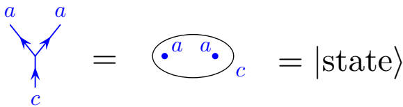
Fig. 10.1 Two a particles fusing to a c particle.
