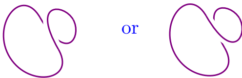
Fig. 22.6 Blow up/ Blow down. Addition or removal of an unlinked loop with a single curl leaves the 3-manifold represented by surgery on the knot unchanged.
