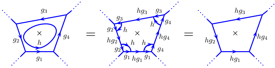
Fig. 29.12 The plaquette operator P_\beta(h) can be viewed as inserting a loop labeled h and pushing it into the edges. In going from the left to the middle we use Fig. ?? once on each edge. The in going from the middle to the right we use Fig. 29.11 once on each corner. The \times in the middle of the plaquette should be thought of as a puncture in the plane. This prevents us from removing the loop using Move 2, but instead forces us to merge the loop into the edges.
