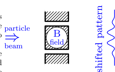
Fig. 4.2 Adding a magnetic field inside the middle box in the Young two slit experiment. Here the circular region includes a constant magnetic field. No magnetic field leaks out of the box. Nonetheless, if the particle being sent into the interferometer is charged, the interference pattern is changed compared to the above figure.
