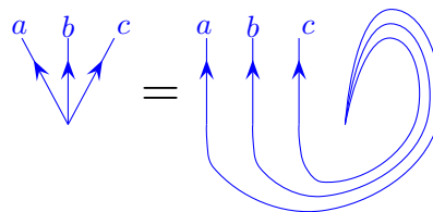
Fig. 14.28 Another version of the pivotal identity. We can derive this from Fig. 14.27 by turning up the c -leg.
