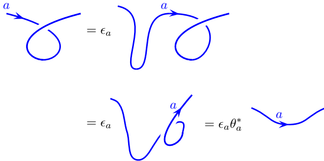
Fig. 15.8 A curl in a rope turned sideways gets a twist factor \theta^* along with a zig-zag factor \epsilon_a . The first step introduces a zig-zag in the curve and we incur a factor of \epsilon_a as in Fig. 14.5. The second step is an allowed smooth deformation (See exercise 15.2). In the last step we remove the curl and obtain a factor of \theta_a^* as in Fig. 15.3. In isotopy invariant cases we have chosen \epsilon_a to be unity.
