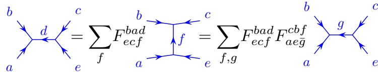
Fig. 16.12 In the second step we apply the same F -matrix equation from Fig. 16.3, but the diagram is rotated by 90 degrees.
