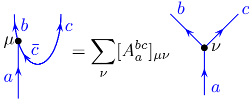
Fig. 14.25 The matrix A_a^{bc} is a unitary matrix in the indices \mu and \nu . In the simpler case of Fig. 14.18, the prefactor is a unitary one-by-one matrix, meaning it is a magnitude one complex scalar.
