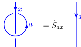
Fig. 17.2 The locality principle tells us that the value of a loop of a around a world line x is some number which we call \tilde{S}_{ax} . (Indeed, we can use the R -matrix to calculate \tilde{S}_{ax} . See exercise 17.4.)
