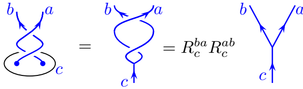
Fig. 13.4 A double exchange is a full braid (one particle wrapping fully around another). If you read two R matrices in right to left order, they are implemented top to bottom.
