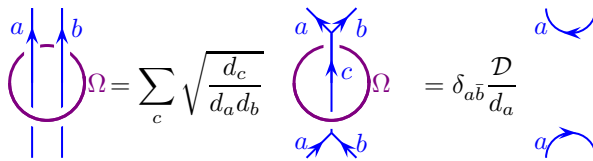
Fig. 17.9 The \Omega -strand joins two lines due to the killing property which we use in the second step to force c to be the identity.
