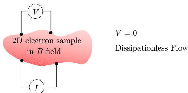
Fig. 2.14 Measurement of longitudinal resistance in FQHE experiment.
