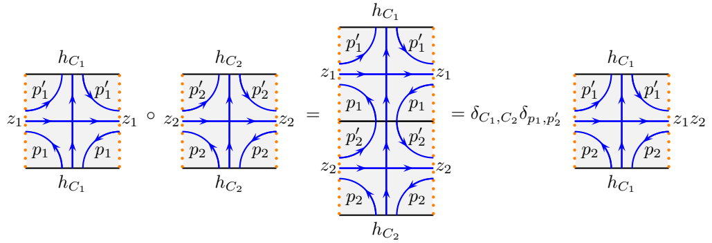
Fig. 29.18 Graphical demonstration of the composition law Eq. 29.17.
