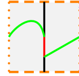
Fig. 30.9 Lines on a torus. If we let our lines follow the colored paths on the torus, our basis states will have the same number of caps as the basis states when written on the annulus
