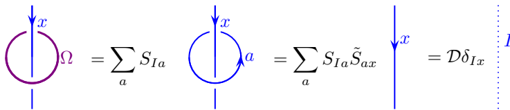
Fig. 17.8 The killing property of the \Omega -strand for modular theories. A loop of Kirby color ( \Omega ) allows no particles through it except the identity. In the final step we use unitarity of S (and the fact that S_{Ia} = S_{Ia}^* ).
