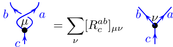
Fig. 13.13 Definition of R -matrix when there are higher fusion multiplicities. Here the vertices carry labels, and R is a unitary matrix with respect to these labels.
