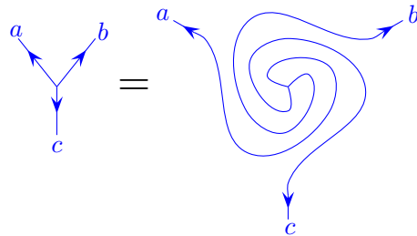
Fig. 14.27 The pivotal identity
