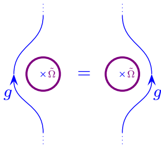
Fig. 29.25 The planar handle-slide.
