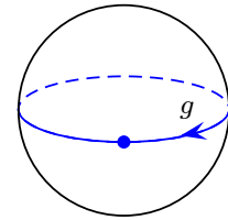
Fig. 29.7 This is the minimal lattice decomposition of a sphere. It consists of a single vertex, a single edge (labeled g ) and two plaquettes — one covering the north hemisphere and one covering the south hemisphere.
