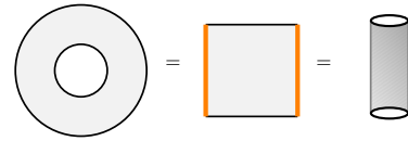
Fig. 28.6 Three different representations of (things topologically equivalent to) the annulus. In the middle figure the two orange sides are identified with each other.
