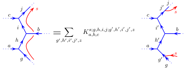
Fig. 31.20 Final result of absorbing a string under the lattice into the lattice.
