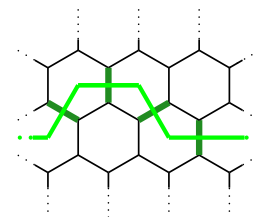
Fig. 30.2 In the doubled semion model, the magnetic string operator applies \sigma_z to the dark green edges which cut through the bright green path on the dual lattice.
