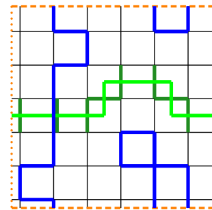
Fig. 25.15 If a string of \sigma_z goes around a cycle (in this case the horizontal cycle), it measures the parity of the number of blue strings going around the opposite cycle (in this case looping in the vertical direction). In this figure, the string of \sigma_z operators returns an end result of -1 being that it cuts an odd number of blue edges.
