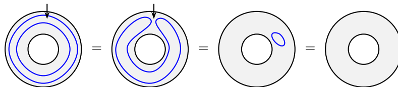
Fig. 28.8 Two loops around the annulus can be covered to no loops by using the moves in Fig. 28.3. In the first step a surgery move is used at the position of the arrow. In the second step we have isotopy (smooth deformation). Finally in the last step we have loop removal.
