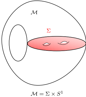
Fig. 7.7 Gluing the top of \Sigma \times I to the bottom we obtain \mathcal{M} = \Sigma \times S^1 . An important fact is that Z(\Sigma \times S^1) is just the ground state degeneracy of the 2-manifold \Sigma
