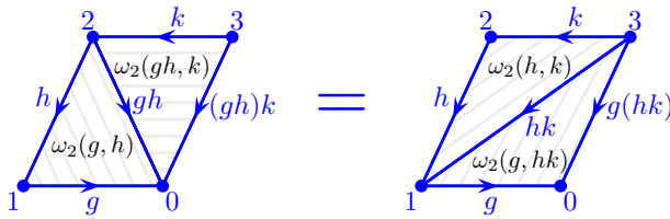
Fig. 21.7 Each triangle satisfies the flatness condition Eq. 21.6 meaning multiplying all three edges in order gives the identity. In the partition function each triangle gets a weight given by the corresponding cocycle \omega_2 as written in black text. All of the triangles in the figure are oriented positively s = +1 . The cocycle condition Eq. 21.13 guarantees that the product of the cocycles on the left equals the product of the cocycle on the right.
