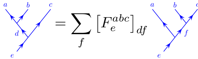
Fig. 12.29 The F -matrix. See chapter 9.
