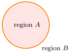
Fig. 33.1 Partititoning a system into two regions.
