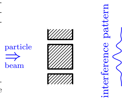
Fig. 4.1 The Young two slit experiment (not to scale).
