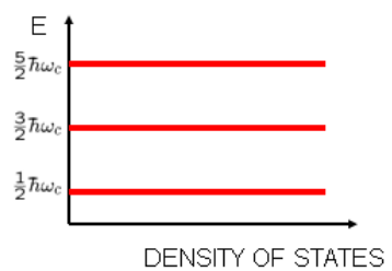
Fig. 35.5 The density of states for spin-polarized (or spinless) electrons in a magnetic field. At energies equal to half-odd integer multiples of the cyclotron frequency, there is a spike of degenerate states, with degeneracy \frac{\text{Area}}{\phi_0} B .
