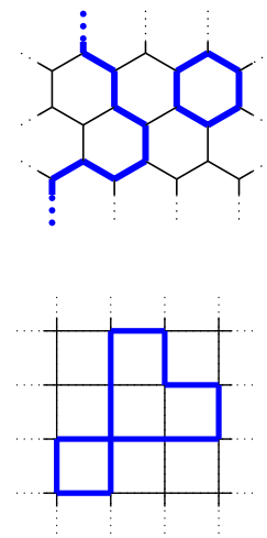
Fig. 28.1 The toric code loop gas can be constructed on any lattice. It is useful to choose a lattice where only three edges meet at a vertex, such as the honeycomb shown on the top. This eliminates the possibility of four lines intersecting at a single corner as shown with the square lattice as shown on the bottom.
