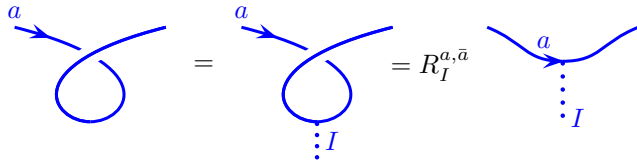
Fig. 15.7 This curl is evaluated with the R matrix. Note that this diagram is not precisely equal to \theta_a^* (See Fig. 15.8).
