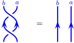
Fig. 20.8 In 3+1 dimensions these two pictures are topologically equivalent. Thus all particles are transparent. This implies Eq. 20.25.
