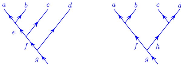
Fig. 12.31 Two (of five) possible bases for describing states of four particles. These bases are related to each other by F -moves (See Fig. 9.7). The shape of tree on the left is sometimes known as the “standard” basis.
