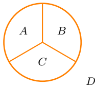
Fig. 33.5 Partititoning a sphere into four regions. The region D includes the remainder of the sphere (i.e., the “point at infinity” for the stereographic projection to the plane).
