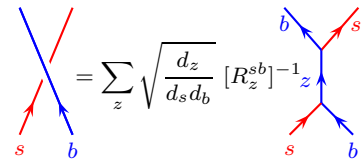
Fig. 31.18 The uncrossing rule. See Fig. 16.19
