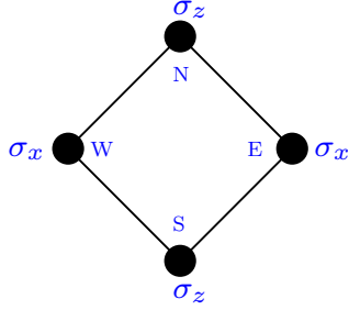
Fig. 32.3 The terms in the Hamiltonian, Eq. 32.2, on every diamond (diamonds of either color in blue in Fig. 32.2) are a product of \sigma_z on the north and south vertices, and \sigma_x on the east and west vertices.
