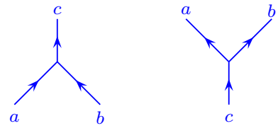
Fig. 14.20 With time going vertical, the left diagram is a negative- d cap if and only if d_a < 0 and d_b < 0 . (The directions of the arrows do not matter, and if the particles are self-dual we do not draw arrows). The right diagram is never a negative- d cap.
