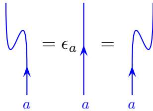
Fig. 14.5 The modified zig-zag identity. Here \epsilon_a is always arranged to be +1 or -1. The equality on the left is from Fig. 14.4. The equality on the right follows from Hermitian conjugation of the equality on the left (turning the diagrams upside down and reversing the arrows).
