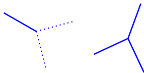
Fig. 18.6 An allowed fusion vertex (right) and a disallowed fusion vertex (left) for the Fibonacci fusion rules. The solid line is \tau and the dotted line is the identity. The vertices shown in Fig. 18.2 are also allowed.
