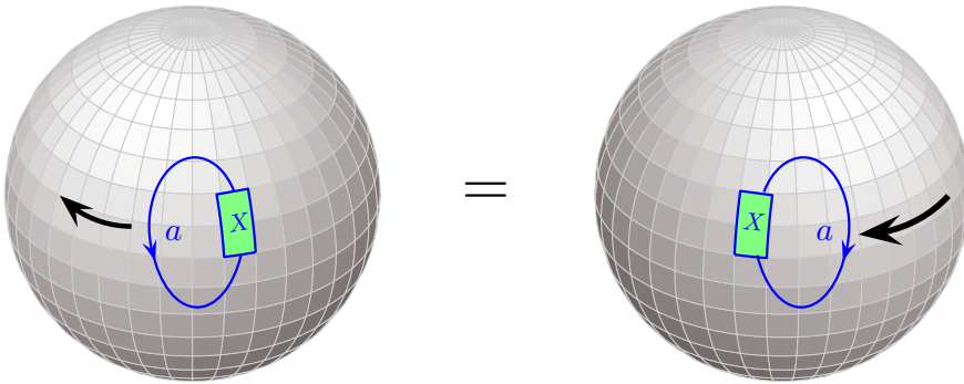
Fig. 14.30 The naming “spherical” comes from the idea that we can pull the string around the back of a sphere (as indicated by the black arrows) to turn a left trace into a right trace.
