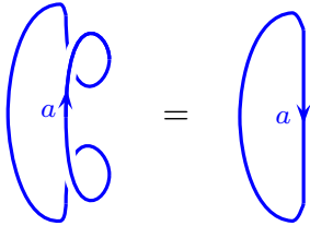
Fig. 15.4 This equality establishes \theta_a \theta_a^* = 1 , hence |\theta_a| = 1 . We can evaluate the diagram on the left by removing the two curls and getting \theta_a \theta_a^* times the diagram on the right. On the other hand, the diagram on the left can also be turned directly into that on the right just by using moves which we know are allowed such as Fig. 13.9. (See also exercise 15.2).
