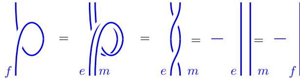
Fig. 26.4 The f particle is a fermion since its twist factor is \theta_f = -1 . We can derive this by using f = e \times m and using the fact that e braiding around m gives a -1 sign.
