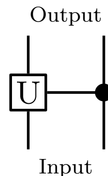
Fig. 11.9 Typical notation for a controlled unitary gate C(U) . The second qubit controls the first.
