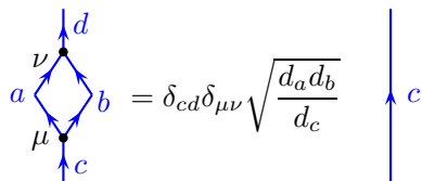
Fig. 14.31 The bubble diagram when there are fusion multiplicities. This diagram is drawn in the isotopy invariant normalization. Compare to Fig. 12.39.
