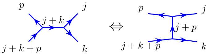
Fig. 28.19 This is the caption. Compare Fig. 28.3
