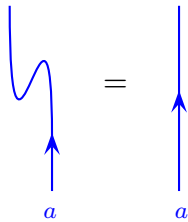
Fig. 16.2 For the isotopy invariant theories considered in this chapter, this deformation is allowed.
