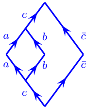
Fig. 14.22 An example of a diagram which should have a positive definite value since it can be written as \langle \text{state} | \text{state} \rangle .
