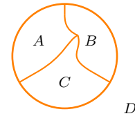
Fig. 33.7 Changing the region near the triple intersection of A , B , and C . The other three triple intersections are assumed to be unchanged, as are all boundaries with region D .
