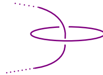
Fig. 22.5 A circumcision. Both strings can be removed. This is a third Kirby move which is implied by the first two if you start with a link embedded in S^3 but is more generally an independent move that is required. See for example Roberts [1997].
