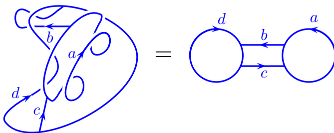
Fig. 16.1 For a theory with full isotopy invariance (regular isotopy invariance) these two diagrams must evaluate to the same result since one can be continuously deformed into the other treating the lines as ribbons.
