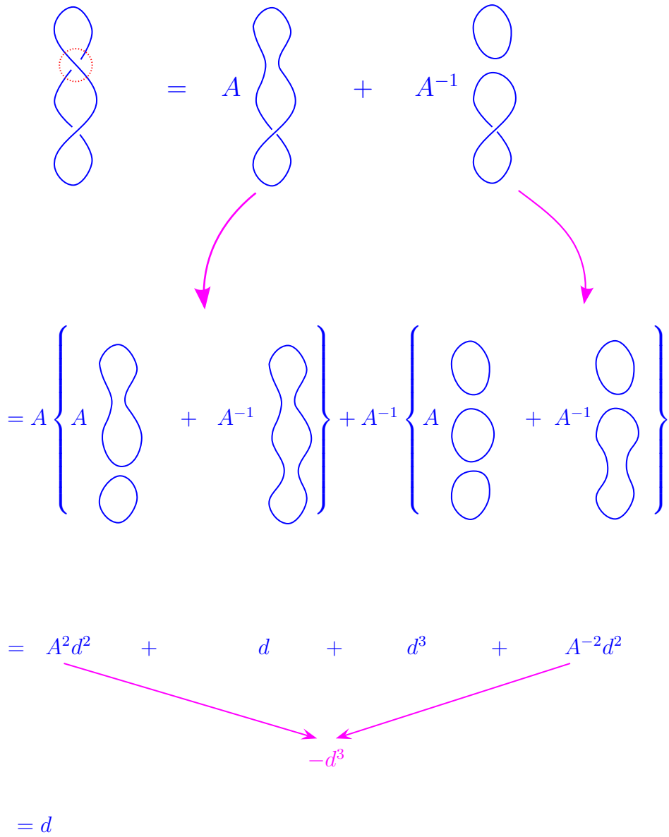
Fig. 2.4 Example of evaluation of the Kauffman bracket invariant for the simple twisted loop in the upper left. The light dotted red circle is meant to draw attention to where we apply the Kauffman crossing rule (the middle line in Fig. 2.3) to get the two diagrams on the right hand side. After applying the Kauffman rules again (the final line in Fig. 2.3), we have removed all crossings and we are left only with simple loops, which each get the value d . In the penultimate line we have used the definition of d to replace A^2 + A^{-2} = -d . The fact that we get d in the end of the calculation is expected since we know that the original knot is just a simple loop (the so-called “unknot”) and the Kauffman rules tell us that a loop gets a value d .
