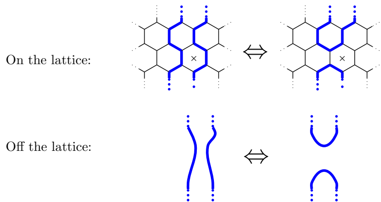
Fig. 28.3 The moves we can make by flipping over a plaquette on the lattice, and their interpretation in the continuum off the lattice. In the diagrams on the lattice, each move is achieved by flipping over the plaquette marked with \times .
