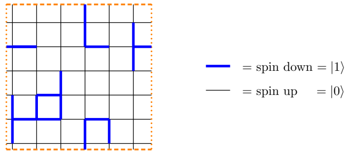
Fig. 25.2 A particular basis state of the Hilbert space, working in the up-down basis ( \sigma_z -eigenstates). Here we denote down spins by thick (blue) lines. Up spins are denoted by not uncolored edges (black).
