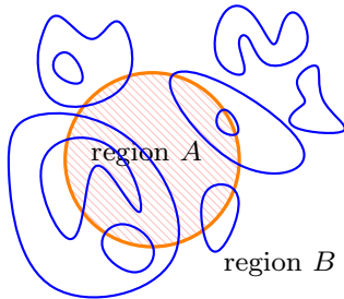
Fig. 33.2 In a loop gas the number of blue lines that cross the boundary of a simply connected region (such as the orange boundary between region A and B) must be even, since if a loop enters the region, it must also exit the region.
