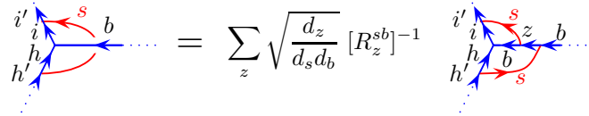
Fig. 31.19 Using the undercrossing rule (Fig. 31.18).
