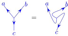
Fig. 16.23 This is an allowed identity in isotopy invariant theories. (Compare the more general Fig. 14.26.
