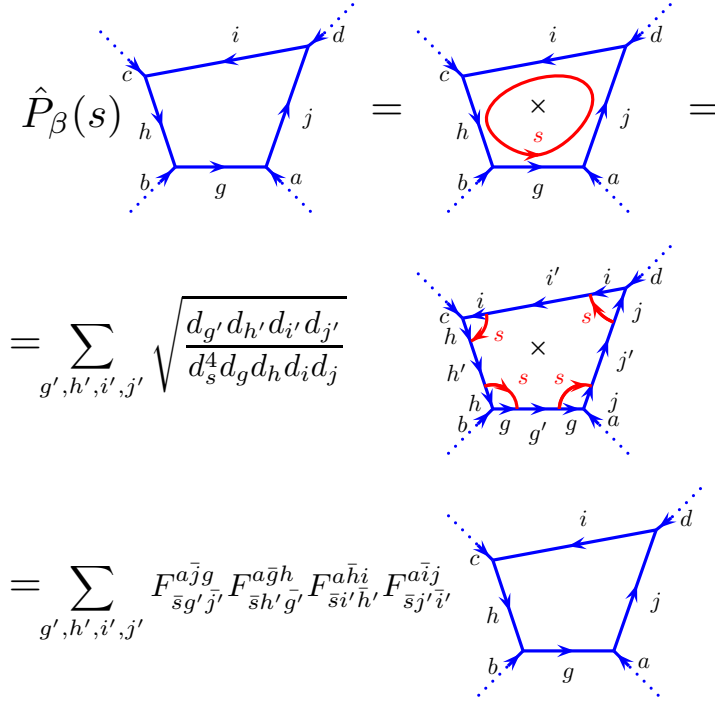
Fig. 31.16 Expressing the plaquette operator as the merging of an s -loop (red) into the edges of the plaquette.
