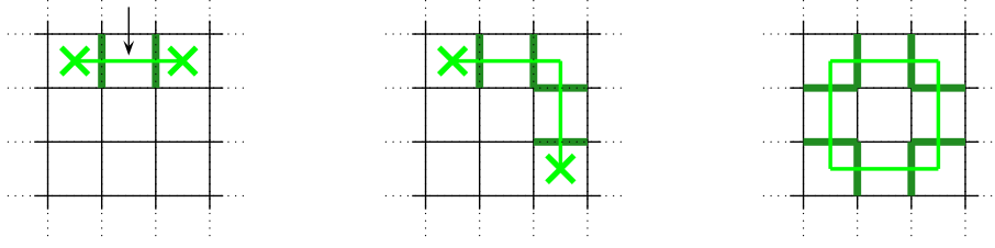
Fig. 25.14 Left: When two \sigma_z operators (dark green) are applied to two different edges of the same plaquette (the one with the arrow) then this plaquette ends up in the P_\beta = +1 state. The two plaquettes with P_\beta = -1 are marked with the bright green \times and are connected together by the bright green error string. Middle: A string of several \sigma_z errors. The bright green line cuts through each of the dark green edges where \sigma_z is applied. The bright green line lives on the dual lattice, meaning it goes from plaquette center to plaquette center. Right: A closed loop of \sigma_z errors. This is equal to the product of all of the enclosed V_\alpha operators. In the code space, this product is equal to +1 .
