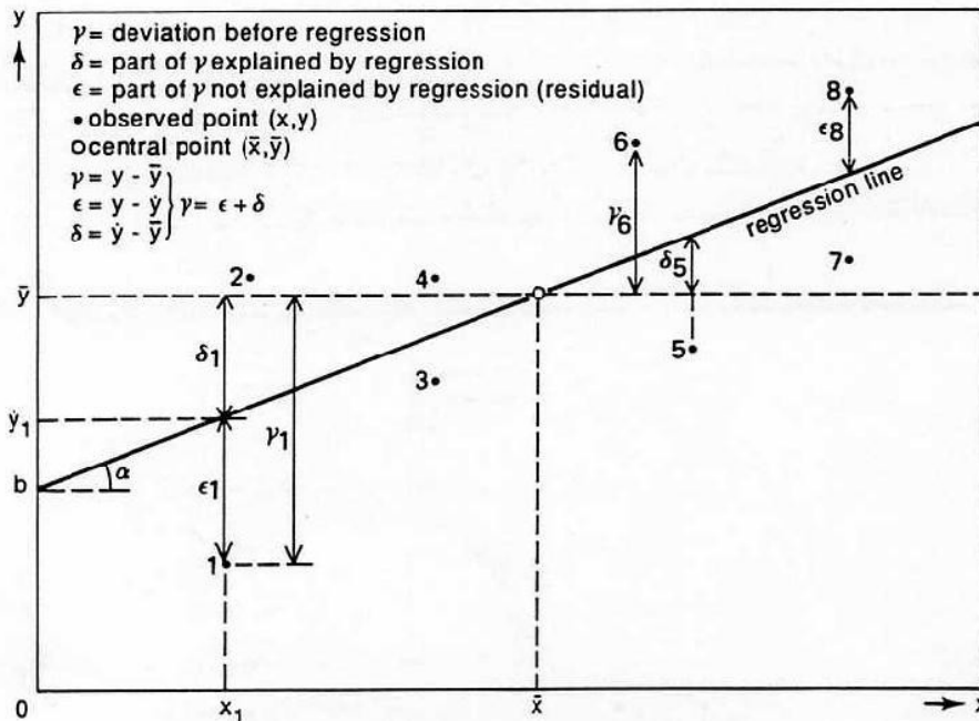
Figure 6.19 Variations in the y-direction
