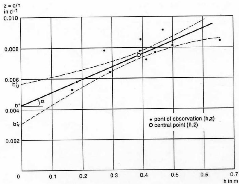
Figure 6.22 Two-way regression with the data of Table 6.12
