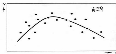
Figure 6.20 A clear relation between y and x , although r \approx 0
