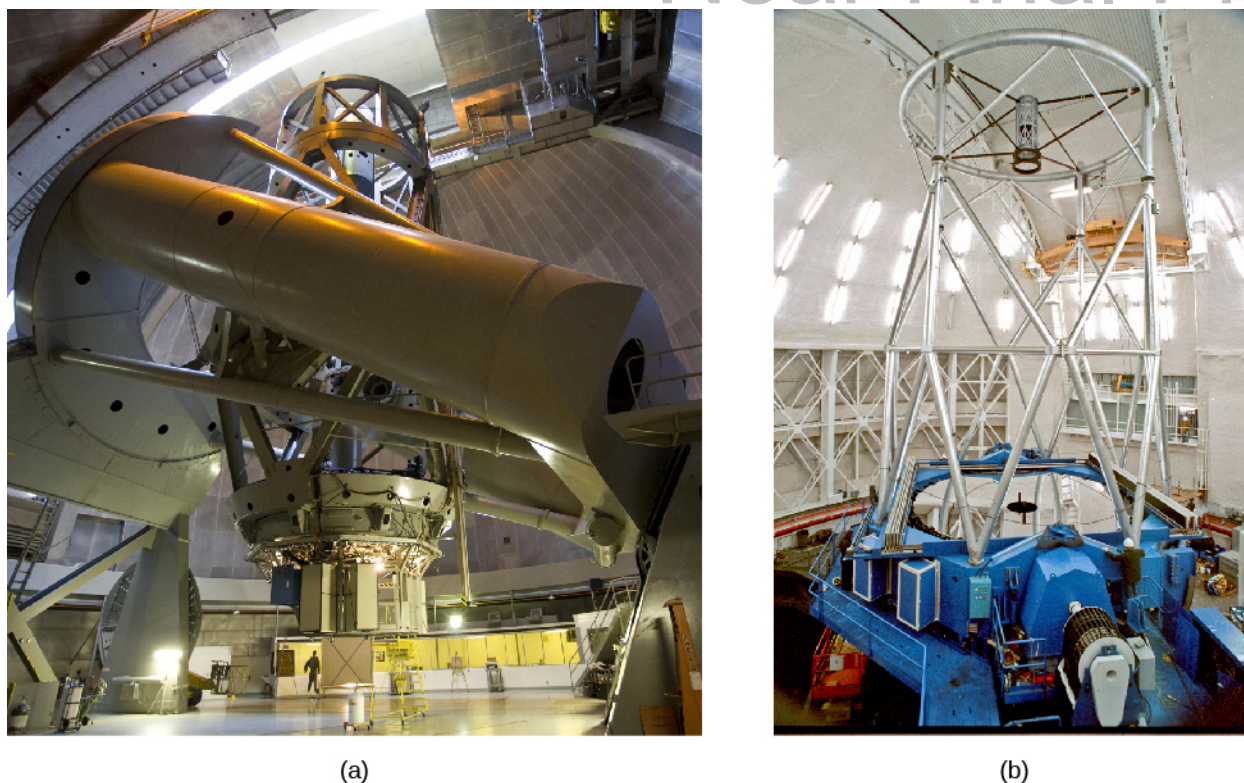
Figure 6.8. Modern Reflecting Telescopes. (a) The Palomar 5-meter reflector: The Hale telescope on Palomar Mountain has a complex mounting structure that enables the telescope (in the open “tube” pointing upward in this photo) to swing easily into any position. (b) The Gemini North 8-meter telescope: The Gemini North mirror has a larger area than the Palomar mirror, but note how much less massive the whole instrument seems. (credit a: modification of work by Caltech/Palomar Observatory; credit b: modification of work by Gemini Observatory/AURA)
