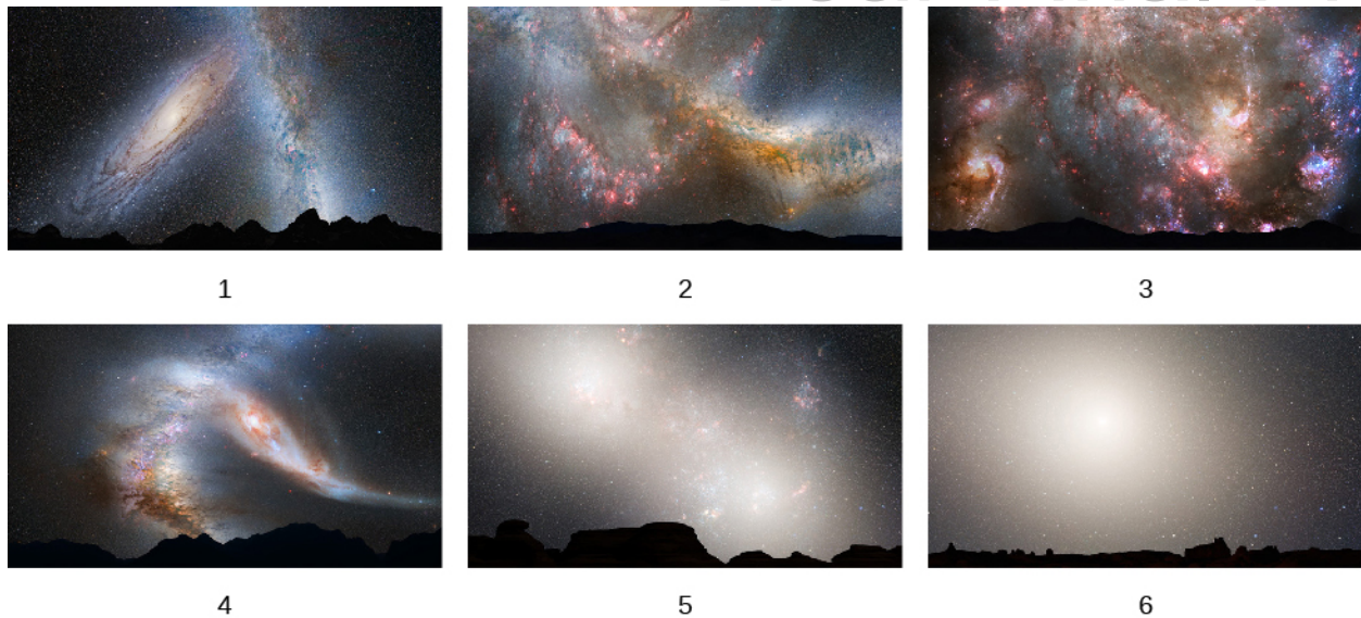
Figure 25.25. Collision of the Milky Way with Andromeda. In about 3 billion years, the Milky Way and the Andromeda galaxies will begin a long process of colliding, separating, and then coming back together to form an elliptical galaxy. The whole interaction will take 3 to 4 billion years. These images show the following sequence: (1) In 3.75 billion years, Andromeda has approached the Milky Way. (2) New star formation fills the sky 3.85 billion years from now. (3) Star formation continues at 3.9 billion years. (4) The galaxy shapes change as they interact, with Andromeda being stretched and our Galaxy becoming warped, about 4 billion years from now. (5) In 5.1 billion years, the cores of the two galaxies are bright lobes. (6) In 7 billion years, the merged galaxies form a huge elliptical galaxy whose brightness fills the night sky. This artist's illustrations show events from a vantage point 25,000 light-years from the center of the Milky Way. However, we should mention that the Sun may not be at that distance throughout the sequence of events, as the collision readjusts the orbits of many stars within each galaxy. (credit: NASA; ESA; Z. Levay, R. van der Marel, STScI; T. Hallas, and A. Mellinger)
