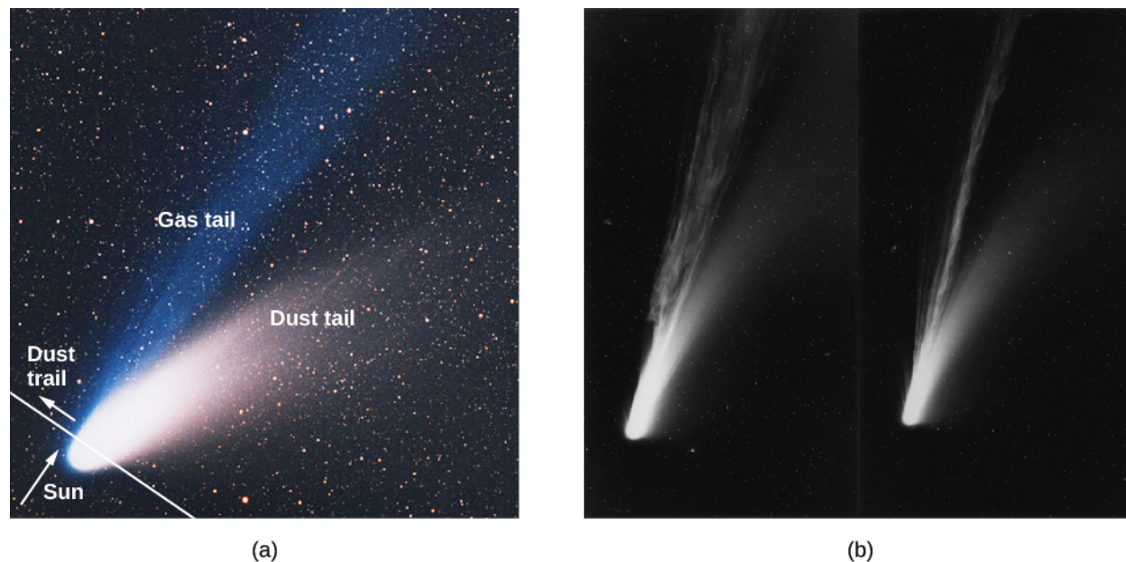
Figure 13.23. Comet Hale-Bopp's Tails. (a) As a comet nears the Sun, its features become more visible. In this illustration from NASA, you can see a comet's two tails: the more easily visible dust tail, which can be up to 10 million kilometers long, and the fainter gas tail (or ion tail), which is up to hundreds of millions of kilometers long. The grains that make up the dust tail are the size of smoke particles. (b) Comet Mrkos was photographed in 1957 with a wide-field telescope at Palomar Observatory and also shows a clear distinction between the straight gas tail and the curving dust tail. (credit a: modification of work by ESO/E. Slawik; credit b: modification of work by Charles Kearns, George O. Abell, and Byron Hill)
