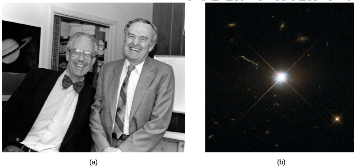
Figure 27.3. Caption: Quasar Pioneers and Quasar 3C 273. (a) Maarten Schmidt (left), who solved the puzzle of the quasar spectra in 1963, shares a joke in this 1987 photo with Allan Sandage, who took the first spectrum of a quasar. Sandage was also instrumental in measuring the value of Hubble's constant. (b) This is the first quasar for which a redshift was measured. The redshift showed that the light from it took about 2.5 billion years to reach us. Despite this great distance, it is still one of the quasars closest to the Milky Way Galaxy. Note also the faint streak going toward the upper left from the quasar. Some quasars, like 3C 273, eject super-fast jets of material. The jet from 3C 273 is about 200,000 light-years long. (credit b: modification of work by ESA/Hubble/NASA)
