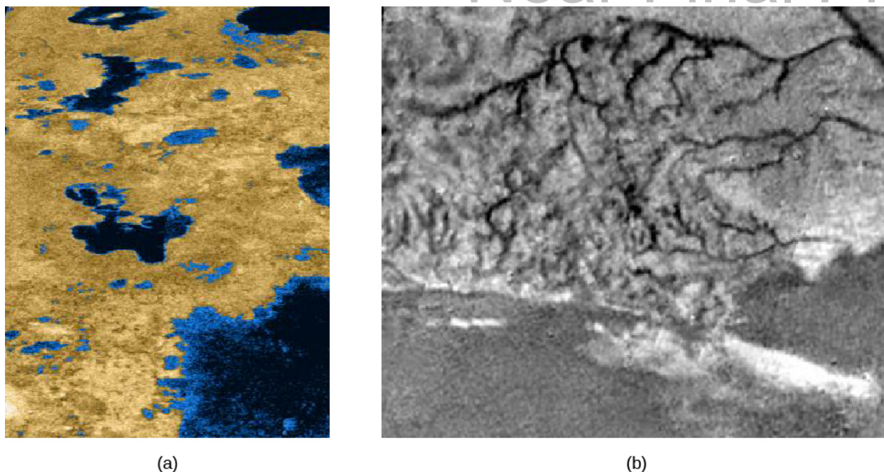
Figure 12.14. Titan's Lakes. (a) This Cassini image from a September 2006 flyby shows the liquid lakes on Titan. Their composition is most likely a combination of methane and ethane. (Since this is a radar image, the colors are artificially added. The dark blue areas are the smooth surfaces of the liquid lakes, and yellow is the rougher solid terrain around them.) (b) This mosaic of Titan's surface from the Cassini-Huygens mission shows in detail a high ridge area and many narrow, sinuous erosion channels that appear to be part of a widespread network of "rivers" carved by flowing hydrocarbons. (credit a: modification of work by NASA/JPL-Caltech/USGS; credit b: modification of work by NASA/JPL/ESA/University of Arizona)
