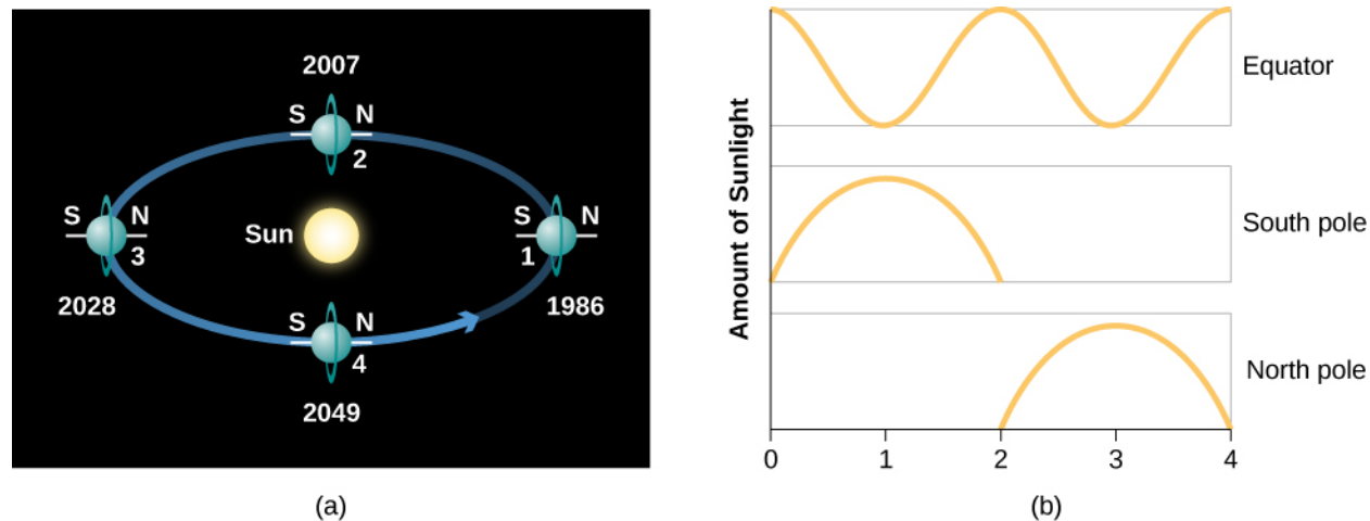
Figure 11.6. Strange Seasons on Uranus. (a) This diagram shows the orbit of Uranus as seen from above. At the time Voyager 2 arrived (position 1), the South Pole was facing the Sun. As we move counterclockwise in the diagram, we see the planet 21 years later at each step. (b) This graph compares the amount of sunlight seen at the poles and the equator of Uranus over the course of its 84-year revolution around the Sun.
