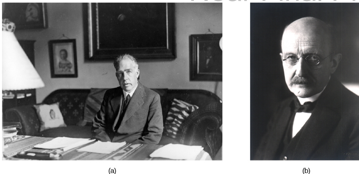
Figure 5.18. Niels Bohr (1885–1962) and Max Planck (1858–1947). (a) Bohr, shown at his desk in this 1935 photograph, and (b) Planck helped us understand the energy behavior of photons.
