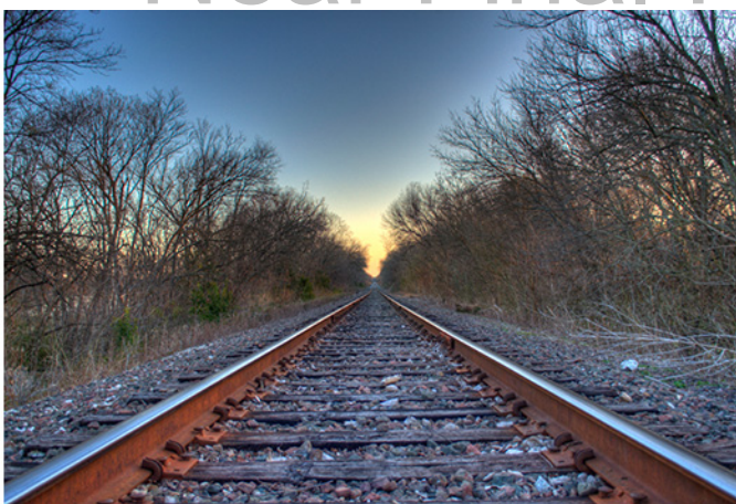
Figure 14.3. Radiant of a Meteor Shower. The tracks of the meteors diverge from a point in the distance, just as long, parallel railroad tracks appear to do. (credit “tracks”: Nathan Vaughn)
