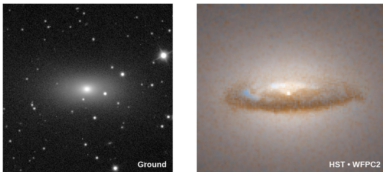
Figure 27.9. Another Galaxy with a Black-Hole Disk. The ground image shows an elliptical galaxy called NGC 7052 located in the constellation of Vulpecula, almost 200 million light-years from Earth. At the galaxy's center (right) is a dust disk roughly 3700 light-years in diameter. The disk rotates like a giant merry-go-round: gas in the inner part (186 light-years from the center) whirls around at a speed of 155 kilometers per second (341,000 miles per hour). From these measurements and Kepler's third law, it is possible to estimate that the disk is orbiting around a central black hole with a mass of 300 million Suns. (credit: modification of work by Roeland P. van der Marel (STScI), Frank C. van den Bosch (University of Washington), NASA)
