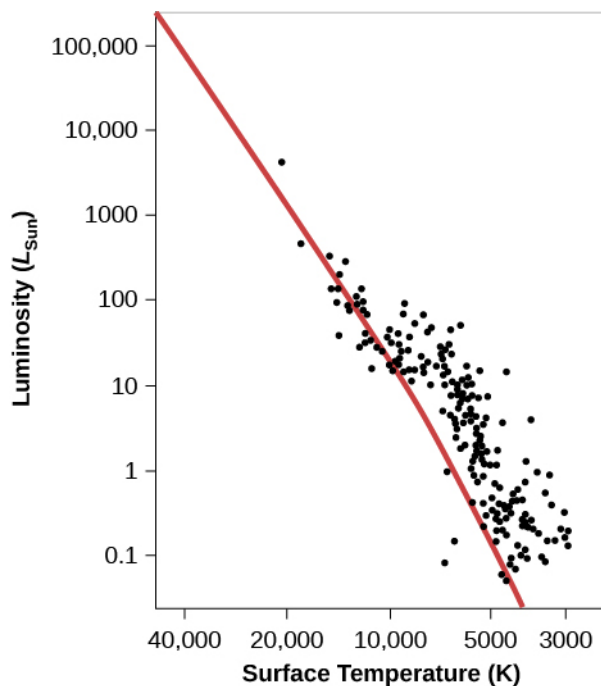
Figure 22.8. NGC 2264 H-R Diagram. Compare this H-R diagram to that in Figure 22.6 ; although the points scatter a bit more here, the theoretical and observational diagrams are remarkably, and satisfyingly, similar.
