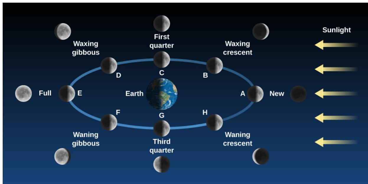
Figure 4.14. Phases of the Moon. The appearance of the Moon changes over the course of a complete monthly cycle. The circle showing the Moon’s orbit shows a perspective from space, with the Sun off to the right in a fixed position. Imagine yourself standing on Earth, facing the Moon in each part of its orbit around Earth. In the position “New,” for example, you are facing the Moon from the right side of Earth in the middle of the day. Next to the image of the orbiting Moon, you can see the appearance of the Moon from Earth as you would see it from each position. (Note that the distance of the Moon from Earth is not to scale in this diagram: the Moon is roughly 30 Earth-diameters away from us.) The outer images show how the Moon appears to you in the sky. (credit: modification of work by NASA)
