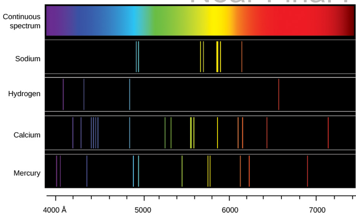
Figure 5.13. Continuous Spectrum and Line Spectra from Different Elements. Each type of glowing gas (each element) produces its own unique pattern of lines, so the composition of a gas can be identified by its spectrum. The spectra of sodium, hydrogen, calcium, and mercury gases are shown here.
