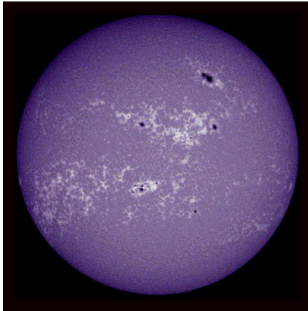
Figure 15.18. Plages on the Sun. This image of the Sun was taken with a filter that transmits only the light of the spectral line produced by singly ionized calcium. The bright cloud-like regions are the plages. (credit: NASA)
