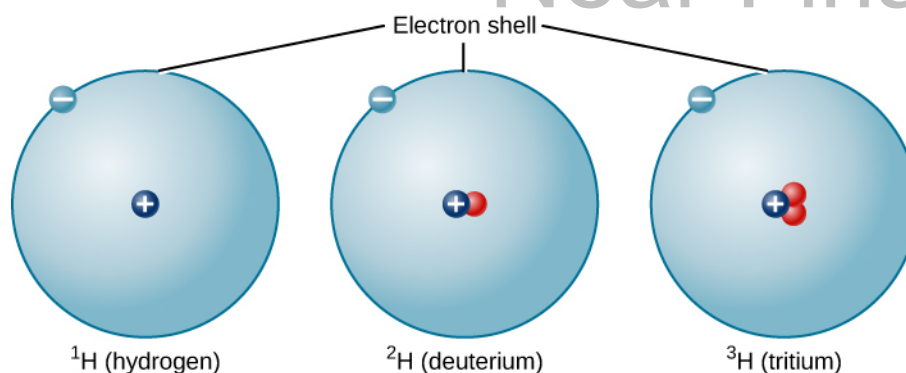
Figure 5.17. Isotopes of Hydrogen. A single proton in the nucleus defines the atom to be hydrogen, but there may be zero, one, or two neutrons. The most common isotope of hydrogen is the one with only a single proton and no neutrons.
