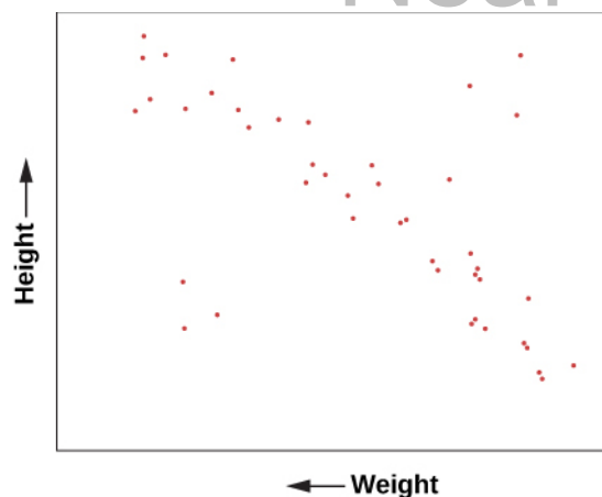
Figure 18.12. Height Versus Weight. The plot of the heights and weights of a representative group of human beings. Most points lie along a “main sequence” representing normal people, but there are a few exceptions.
