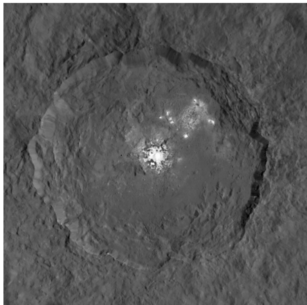
Figure 13.12. White Spots in a Larger Crater on Ceres. These bright features appear to be salt deposits in a crater called Occator, which is 92 kilometers across. (credit: modification of work by NASA/JPL-Caltech/UCLA/MPS/DLR/IDA)
