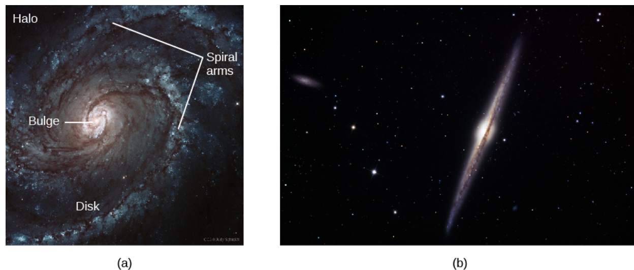
Figure 26.4. Spiral Galaxies. (a) The spiral arms of M100, shown here, are bluer than the rest of the galaxy, indicating young, high-mass stars and star-forming regions. (b) This spiral galaxy, NGC 4565, can be observed from Earth. We view this galaxy almost exactly edge on, and from this angle, we can see the dust in the plane of the galaxy; it appears dark because it absorbs the light from the stars in the galaxy. (credit a: modification of work by Hubble Legacy Archive, NASA, ESA, and Judy Schmidt; credit b: modification of work by "Jschulman555"/ Wikimedia)
