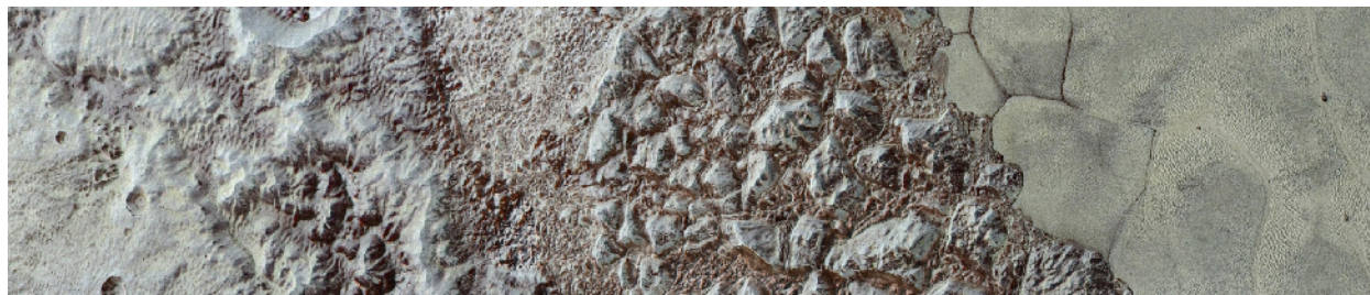
Figure 12.22. Diversity of Terrain on Pluto. This enhanced color view of a strip of Pluto's surface about 80 kilometers long shows a variety of different surface features. From left to right, we first cross a region of “badlands” with some craters showing, and then move across a wide range of mountains made of water ice and coated with the redder material we saw in the previous image. Then, at right, we arrive at the “shoreline” of the great sea of frozen nitrogen that the mission scientists have nicknamed the “Sputnik Plains.” This nitrogen sea is divided into mysterious cells or segments that are many kilometers across. (credit: modification of work by NASA/Johns Hopkins University Applied Physics Laboratory/Southwest Research Institute)
