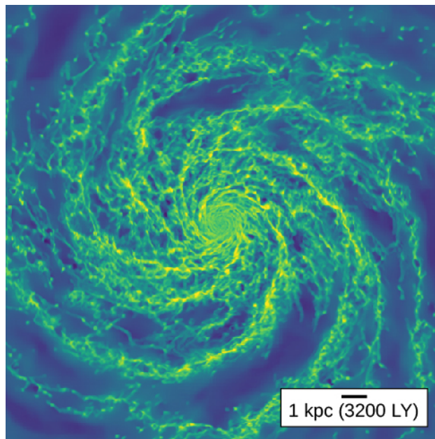
Figure 20.18. Large-Scale Distribution of Interstellar Matter. This image is from a computer simulation of the Milky Way's interstellar medium as a whole. The majority of gas, visible in greenish colors, is neutral hydrogen. In the densest regions in the spiral arms, shown in yellow, the gas is collected into giant molecular clouds. Low-density holes in the spiral arms, shown in blue, are the result of supernova explosions. (credit: modification of work by Mark Krumholz)
