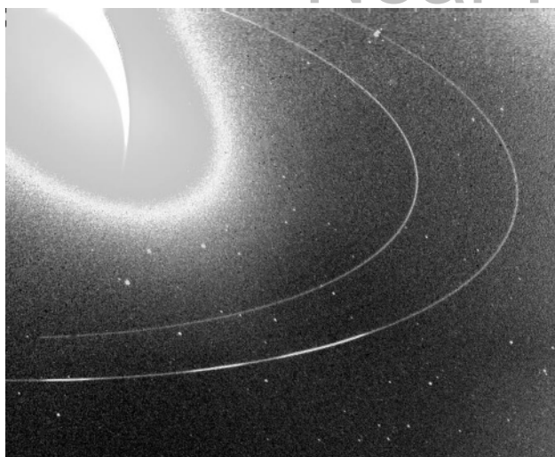
Figure 12.31. Rings of Neptune. This long exposure of the rings of Neptune was photographed by Voyager 2. Note the two denser regions of the outer ring. (credit: modification of work by NASA/JPL)
