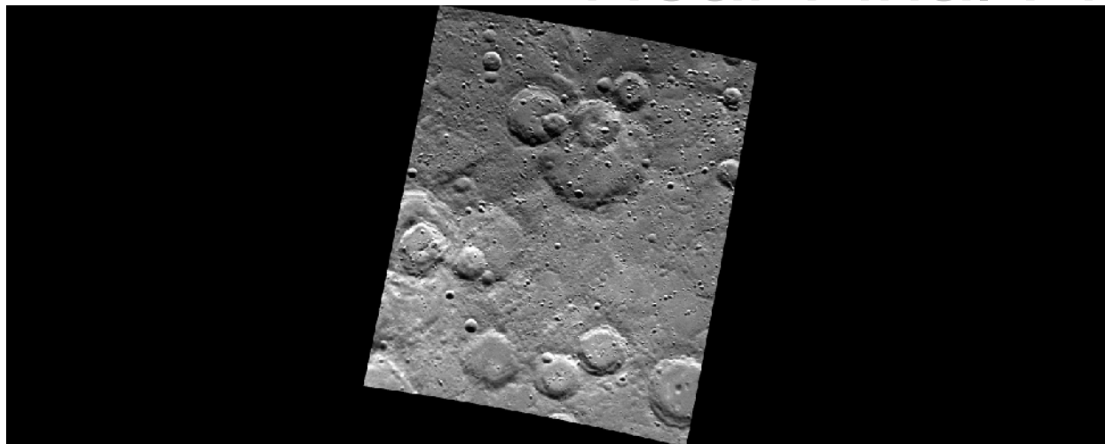
Figure 7.4. Surface of Mercury. The pockmarked face of this terrestrial world is more typical of the inner planets than the watery surface of Earth. This black-and-white image, taken with the Mariner 10 spacecraft, shows a region more than 400 kilometers wide. (credit: NASA/John Hopkins University Applied Physics Laboratory/Carnegie Institution of Washington)
