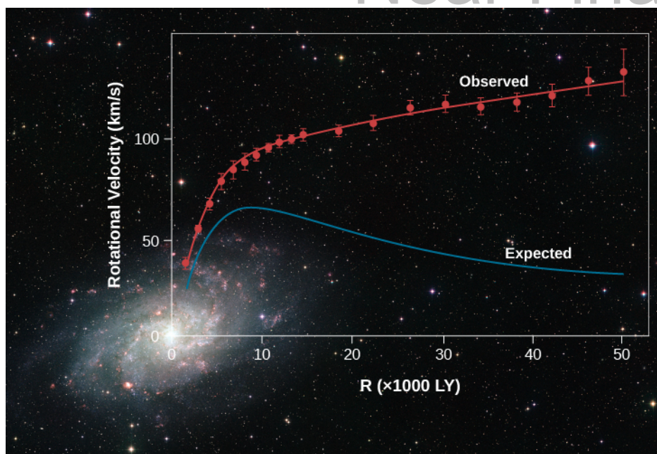
Figure 28.23. Rotation Indicates Dark Matter. We see the Milky Way's sister, spiral galaxy M31, with a graph that shows the velocity at which stars and clouds of gas orbit the galaxy at different distances from the center (red line). As is true of the Milky Way, the rotational velocity (or orbital speed) does not decrease with distance from the center, which is what you would expect if an assembly of objects rotates around a common center. A calculation (blue line) based on the total mass visible as stars, gas, and dust predicts that the velocity should be much lower at larger distances from the center. The discrepancy between the two curves implies the presence of a halo of massive dark matter extending outside the boundary of the luminous matter. This dark matter causes everything in the galaxy to orbit faster than the observed matter alone could explain. (credit background: modification of work by ESO)
