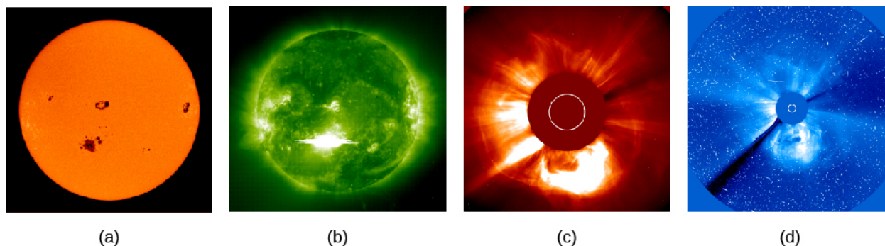
Figure 15.21. A Flare and a Coronal Mass Ejection. This sequence of four images shows the evolution over time of a giant eruption on the Sun. (a) The event began at the location of a sunspot group, and (b) a flare is seen in far-ultraviolet light. (c) Fourteen hours later, a CME is seen blasting out into space. (d) Three hours later, this CME has expanded to form a giant cloud of particles escaping from the Sun and is beginning the journey out into the solar system. The white circle in (c) and (d) shows the diameter of the solar photosphere. The larger dark area shows where light from the Sun has been blocked out by a specially designed instrument to make it possible to see the faint emission from the corona. (credit a, b, c, d: modification of work by SOHO/EIT, SOHO/LASCO, SOHO/MDI (ESA & NASA))
