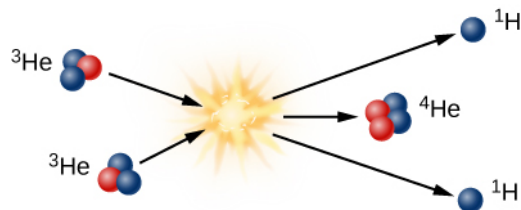
Figure 16.8. Proton-Proton Chain, Step 3. This is the third step in the fusion of hydrogen into helium in the Sun. Note that the two 3-helium nuclei from the second step (see Figure 16.7 ) must combine before the third step becomes possible. The two protons that come out of this step have the energy to collide with other protons in the Sun and start step one again.
