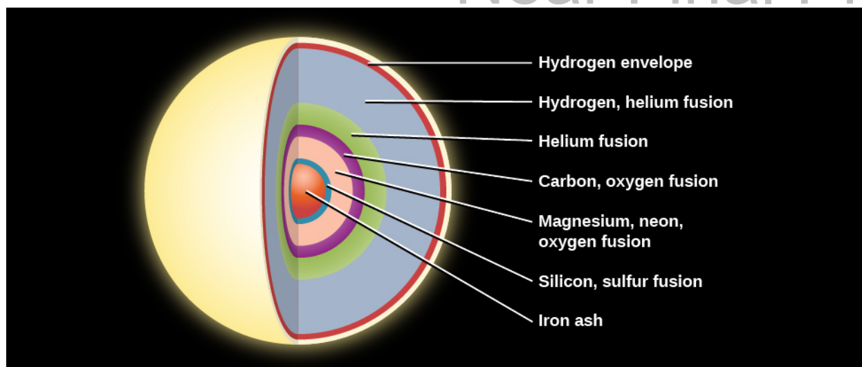
Figure 22.3. Interior Structure of a Massive Star Just before It Exhausts Its Nuclear Fuel. High-mass stars can fuse elements heavier than carbon. As a massive star nears the end of its evolution, its interior resembles an onion. Hydrogen fusion is taking place in an outer shell, and progressively heavier elements are undergoing fusion in the higher-temperature layers closer to the center. All of these fusion reactions generate energy and enable the star to continue shining. Iron is different. The fusion of iron requires energy, and when iron is finally created in the core, the star has only minutes to live.
