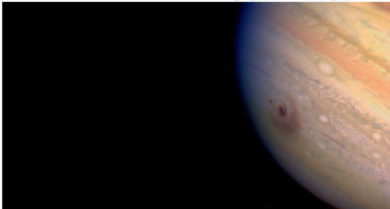
Figure 13.31. Impact Dust Cloud on Jupiter. These features result from the impact of Comet Shoemaker-Levy 9 with Jupiter, seen with the Hubble Space Telescope 105 minutes after the impact that produced the dark rings (the compact back dot came from another fragment). The inner edge of the diffuse, outer ring is about the same size as Earth. Later, the winds on Jupiter blended these features into a broad spot that remained visible for more than a month. (credit: modification of work by H. Hammel, MIT, and NASA/ESA)
