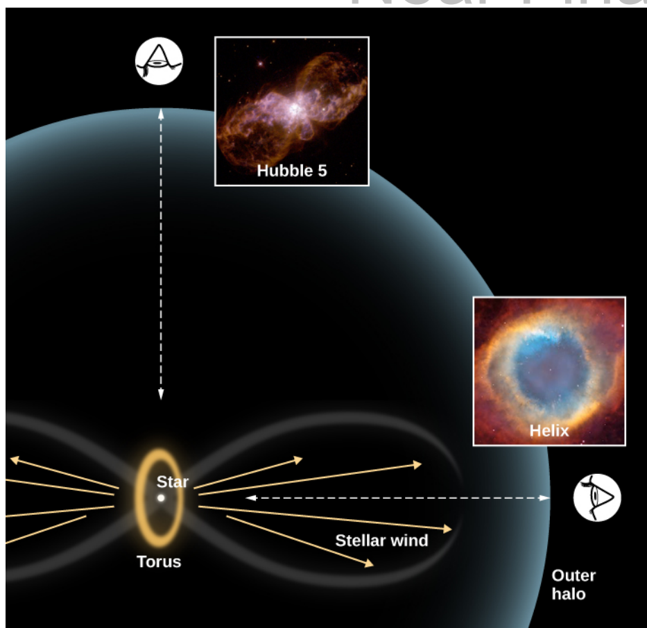
Figure 22.17. Model to Explain the Different Shapes of Planetary Nebulae. The range of different shapes that we see among planetary nebulae may, in many cases, arise from the same geometric shape, but seen from a variety of viewing directions. The basic shape is a hot central star surrounded by a thick torus (or doughnut-shaped disk) of gas. The star's wind cannot flow out into space very easily in the direction of the torus, but can escape more freely in the two directions perpendicular to it. If we view the nebula along the direction of the flow (Helix Nebula), it will appear nearly circular (like looking directly down into an empty ice-cream cone). If we look along the equator of the torus, we see both outflows and a very elongated shape (Hubble 5). Current research on planetary nebulae focuses on the reasons for having a torus around the star in the first place. Many astronomers suggest that the basic cause may be that many of the central stars are actually close binary stars, rather than single stars. (credit "Hubble 5": modification of work by Bruce Balick (University of Washington), Vincent Icke (Leiden University, The Netherlands), Garrelt Mellema (Stockholm University), and NASA/ESA; credit "Helix": modification of work by NASA, ESA, C.R. O'Dell (Vanderbilt University), and M. Meixner, P. McCullough)
