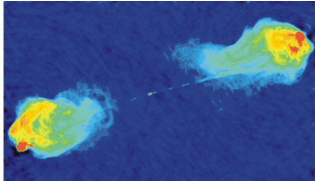
Figure 6.18. Radio Image. This image has been constructed of radio observations of a galaxy called Cygnus A. Colors have been added to help the eye sort out regions of different radio intensities. Red regions are the most intense, blue the least. The visible galaxy would be a small dot in the center of the image. The radio image reveals jets of expelled material (more than 160,000 light-years long) on either side of the galaxy. (credit: "Mhardcastle"/Wikimedia)
