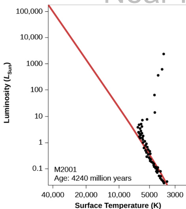
Figure 22.11. H-R Diagram for an Older Cluster. We see the H-R diagram for a hypothetical older cluster at an age of 4.24 billion years. Note that most of the stars on the upper part of the main sequence have now turned off toward the red-giant region.
