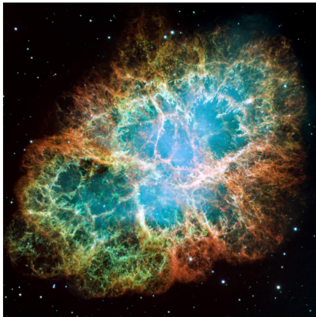
Figure 1.3. A Stellar Corpse. We observe the remains of a star that was seen to explode in our skies in 1054 (and was, briefly, bright enough to be visible during the daytime). Today, the remnant is called the Crab Nebula and its central region is seen here. Such exploding stars are crucial to the development of life in the universe. (credit: NASA, ESA, J. Hester (Arizona State University))
