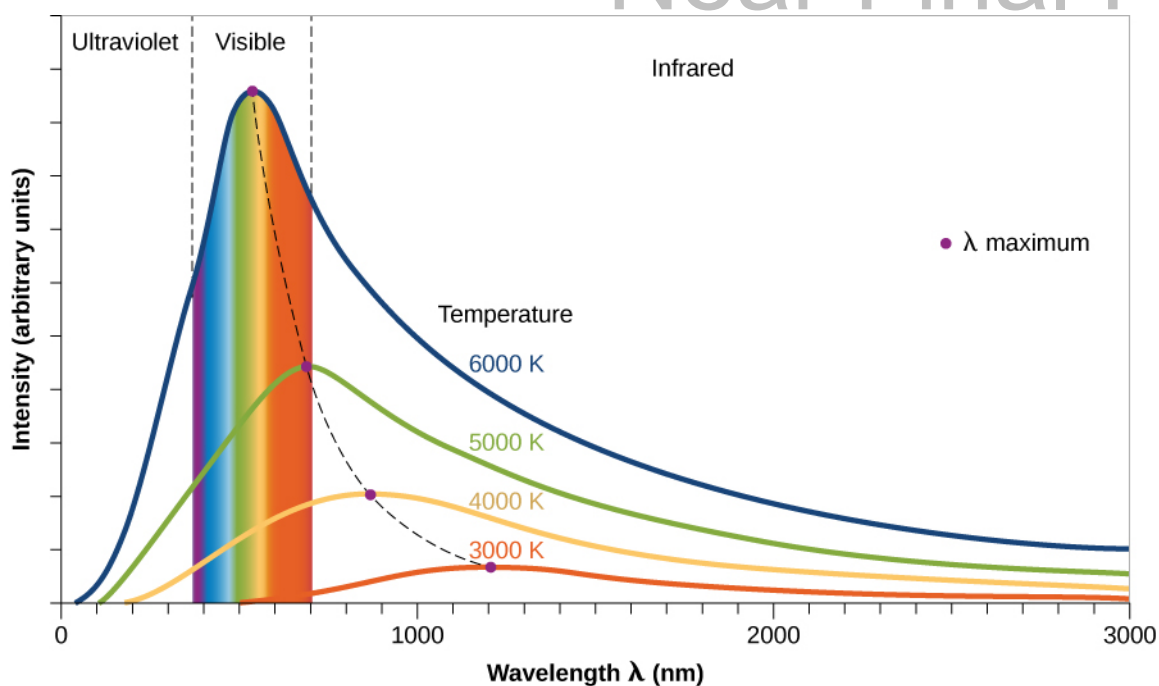
Figure 5.8. Radiation Laws Illustrated. This graph shows in arbitrary units how many photons are given off at each wavelength for objects at four different temperatures. The wavelengths corresponding to visible light are shown by the colored bands. Note that at hotter temperatures, more energy (in the form of photons) is emitted at all wavelengths. The higher the temperature, the shorter the wavelength at which the peak amount of energy is radiated (this is known as Wien's law).
