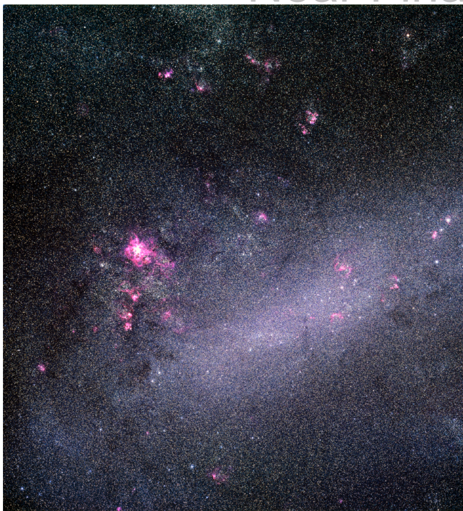
Figure 19.11. Large Magellanic Cloud. The Large Magellanic Cloud (so named because Magellan's crew were the first Europeans to record it) is a small, irregularly shaped galaxy near our own Milky Way. It was in this galaxy that Henrietta Leavitt discovered the cepheid period-luminosity relation. (credit: ESO)
