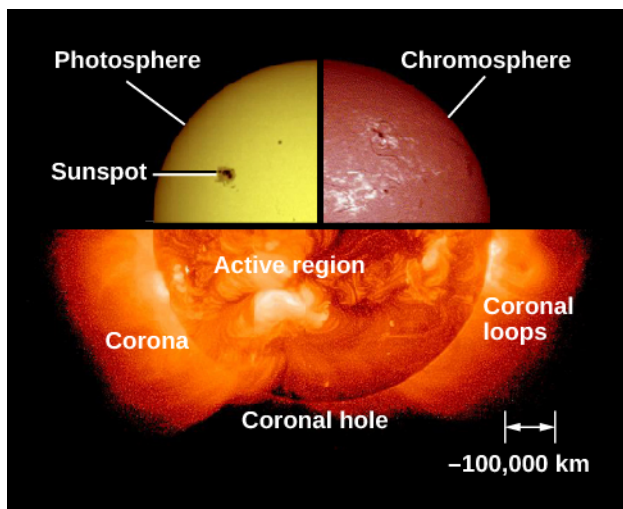
Figure 15.7. The Sun’s Atmosphere. Composite image showing the three components of the solar atmosphere: the photosphere or surface of the Sun taken in ordinary light; the chromosphere, imaged in the light of the strong red spectral line of hydrogen (H-alpha); and the corona as seen with X-rays. (credit: modification of work by NASA)
