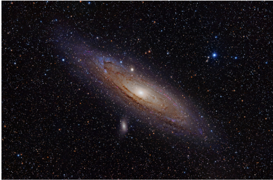
Figure 26.2. Andromeda Galaxy. Also known by its catalog number M31, the Andromeda galaxy is a large spiral galaxy very similar in appearance to, and slightly larger than, our own Galaxy. At a distance of about 2.5 million light-years, Andromeda is the spiral galaxy that is nearest to our own in space. Here, it is seen with two of its satellite galaxies, M32 (top) and M110 (bottom). (credit: Adam Evans)
