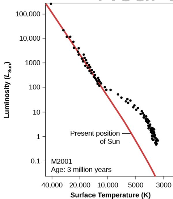
Figure 22.6. Young Cluster H-R Diagram. We see an H-R diagram for a hypothetical young cluster with an age of 3 million years. Note that the high-mass (high-luminosity) stars have already arrived at the main-sequence stage of their lives, while the lower-mass (lower-luminosity) stars are still contracting toward the zero-age main sequence (the red line) and are not yet hot enough to derive all of their energy from the fusion of hydrogen.
