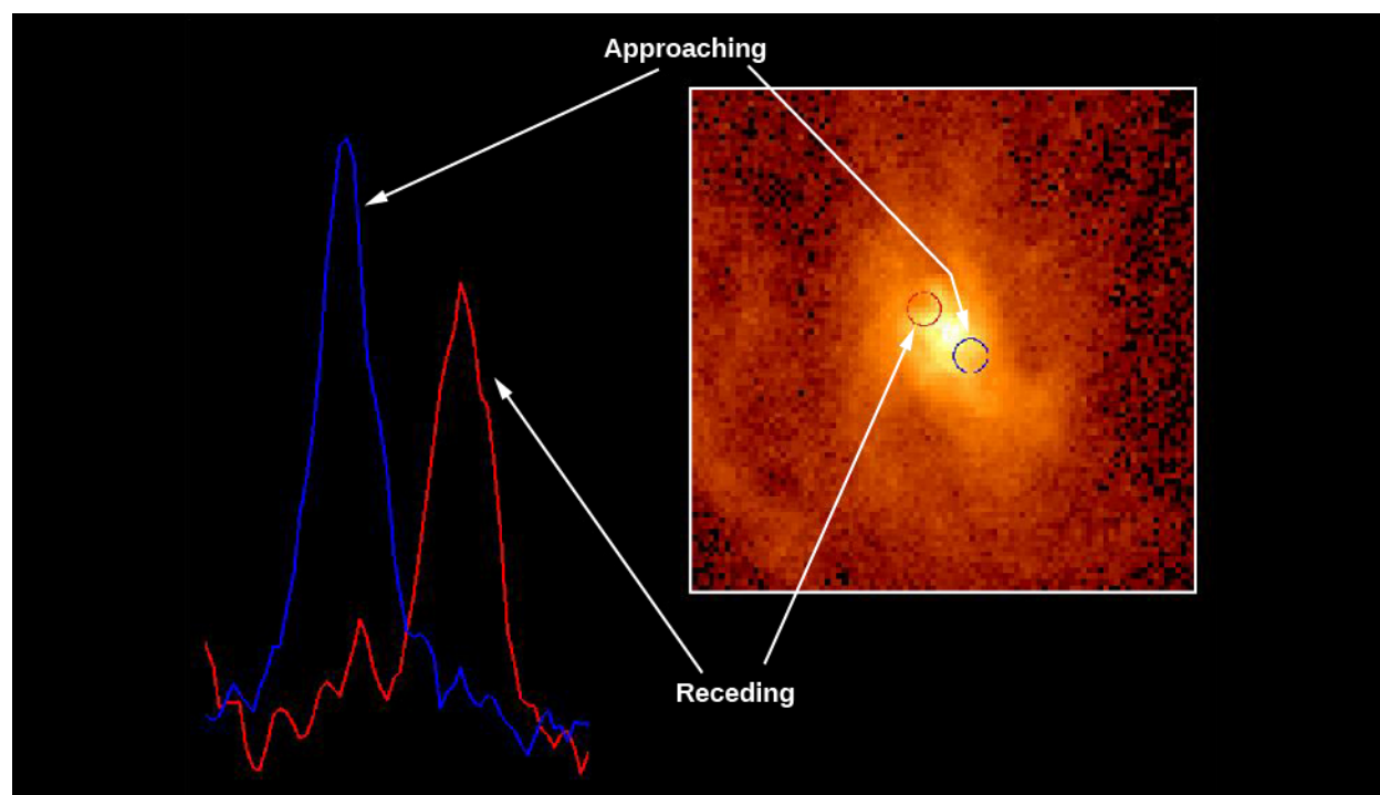
Figure 27.8. Evidence for a Black Hole at the Center of M87. This disk of whirling gas at right was discovered at the center of the giant elliptical galaxy M87 with the Hubble Space Telescope. Observations made on opposite sides of the disk show that one side is approaching us (the spectral lines are blueshifted by the Doppler effect) while the other is receding (lines redshifted), a clear indication that the disk is rotating. The rotation speed is about 550 kilometers per second or 1.2 million miles per hour. Such a high rotation speed is evidence that there is a very massive black hole at the center of M87. (credit: modification of work by Holland Ford, STScI/JHU; Richard Harms, Linda Dressel, Ajay K. Kochhar, Applied Research Corp.; Zlatan Tsvetanov, Arthur Davidsen, Gerard Kriss, Johns Hopkins; Ralph Bohlin, George Hartig, STScI; Bruce Margon, University of Washington in Seattle; NASA)
