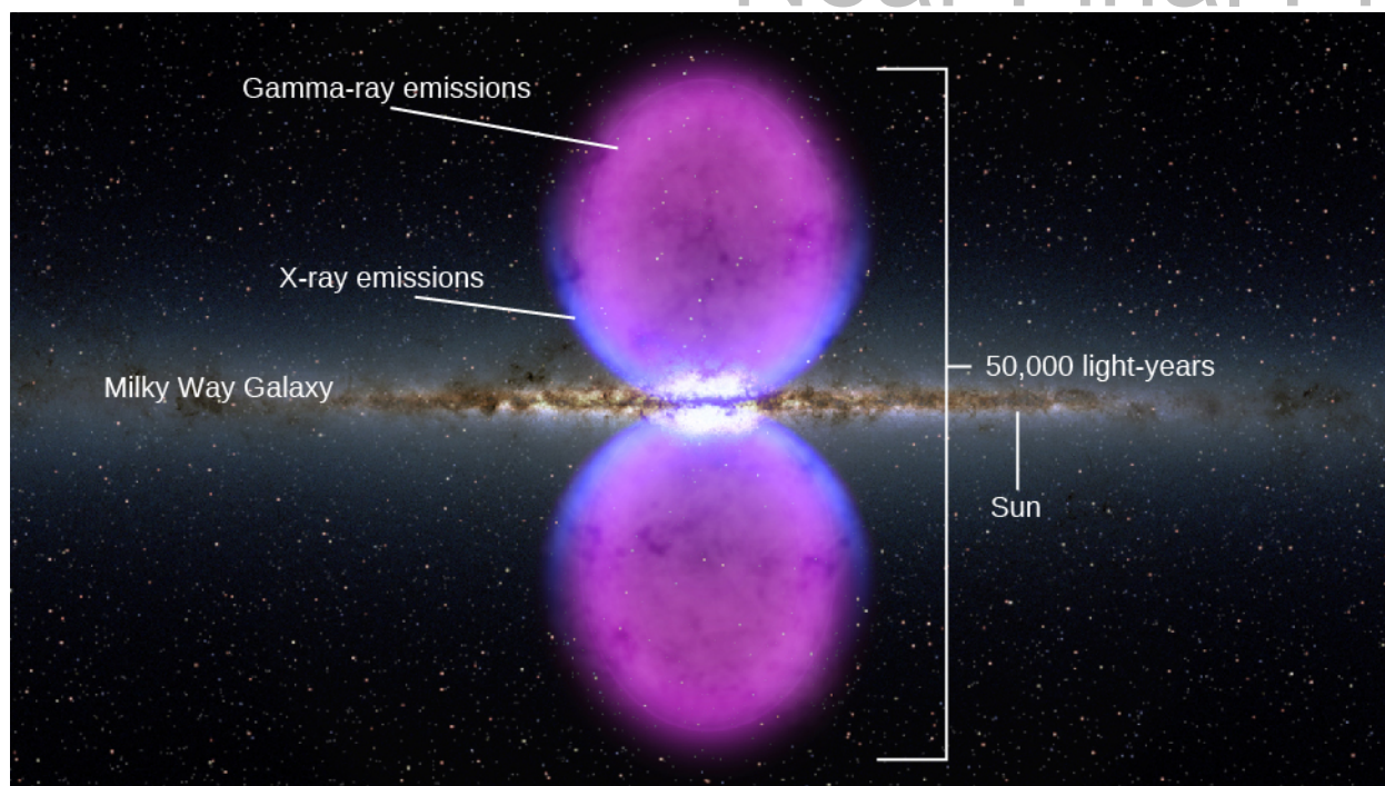
Figure 27.11. Fermi Bubbles in the Galaxy. Giant bubbles shining in gamma-ray light lie above and below the center of the Milky Way, as seen by the Fermi satellite. (The gamma-ray and X-ray image is superimposed on a visible-light image of the inner parts of our Galaxy.) The bubbles may be evidence that the supermassive black hole at the center of our Galaxy was a quasar a few million years ago. (credit: modification of work by NASA's Goddard Space Flight Center)
