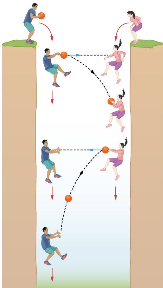
Figure 24.4. Free Fall. Two people playing catch as they descend into a bottomless abyss. Since the people and ball all fall at the same speed, it appears to them that they can play catch by throwing the ball in a straight line between them. Within their frame of reference, there appears to be no gravity.
