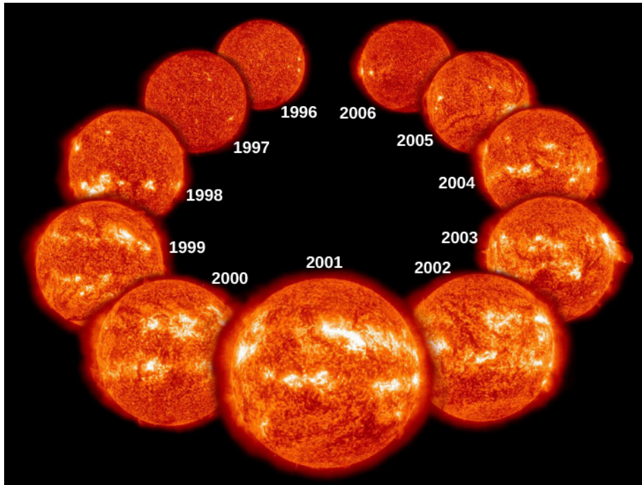
Figure 15.22. Solar Cycle. This dramatic sequence of images taken from the SOHO satellite over a period of 11 years shows how active regions change during the solar cycle. The images were taken in the ultraviolet region of the spectrum and show that active regions on the Sun increase and decrease during the cycle. Sunspots are located in the cooler photosphere, beneath the hot gases shown in this image, and vary in phase with the emission from these hot gases—more sunspots and more emission from hot gases occur together. (credit: modification of work by ESA/NASA/SOHO)
