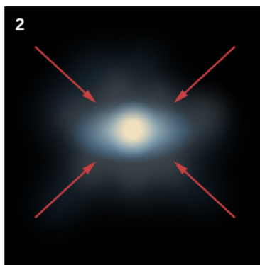
2 Cloud collapses under gravity.
