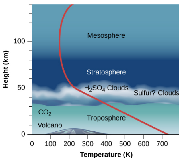
Figure 10.12. Venus' Atmosphere. The layers of the massive atmosphere of Venus shown here are based on data from the Pioneer and Venera entry probes. Height is measured along the left axis, the bottom scale shows temperature, and the red line allows you to read off the temperature at each height. Notice how steeply the temperature rises below the clouds, thanks to the planet's huge greenhouse effect.
