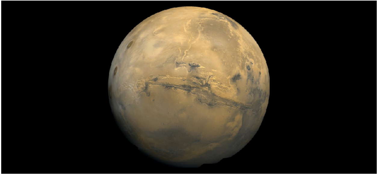
Figure 1.2. Mars Mosaic. This image of Mars is centered on the Valles Marineris (Mariner Valley) complex of canyons, which is as long as the United States is wide. (credit: NASA)
