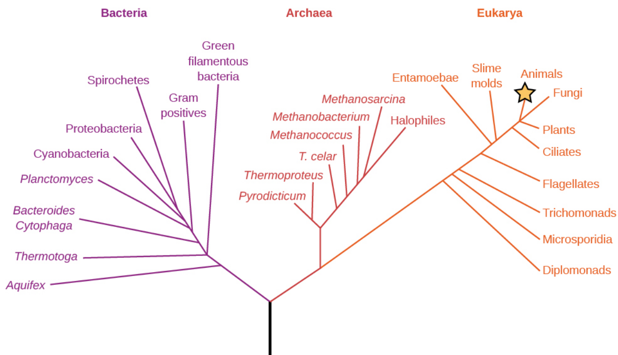
Figure 8.16. Tree of Life. This chart shows the main subdivisions of life on Earth and how they are related. Note that the animal and plant kingdoms are just short branches on the far right, along with the fungi. The most fundamental division of Earth's living things is onto three large domains called bacteria, archaea, and eukarya. Most of the species listed are microscopic. (credit: modification of work by Eric Gaba)
