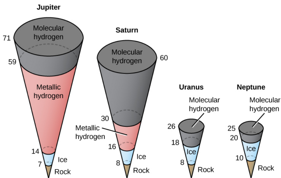
Figure 11.7. Internal Structures of the Jovian Planets. Jupiter and Saturn are composed primarily of hydrogen and helium, but Uranus and Neptune consist in large part of compounds of carbon, nitrogen, and oxygen. (The diagrams are drawn to scale; numbers show radii in thousands of kilometers.)
