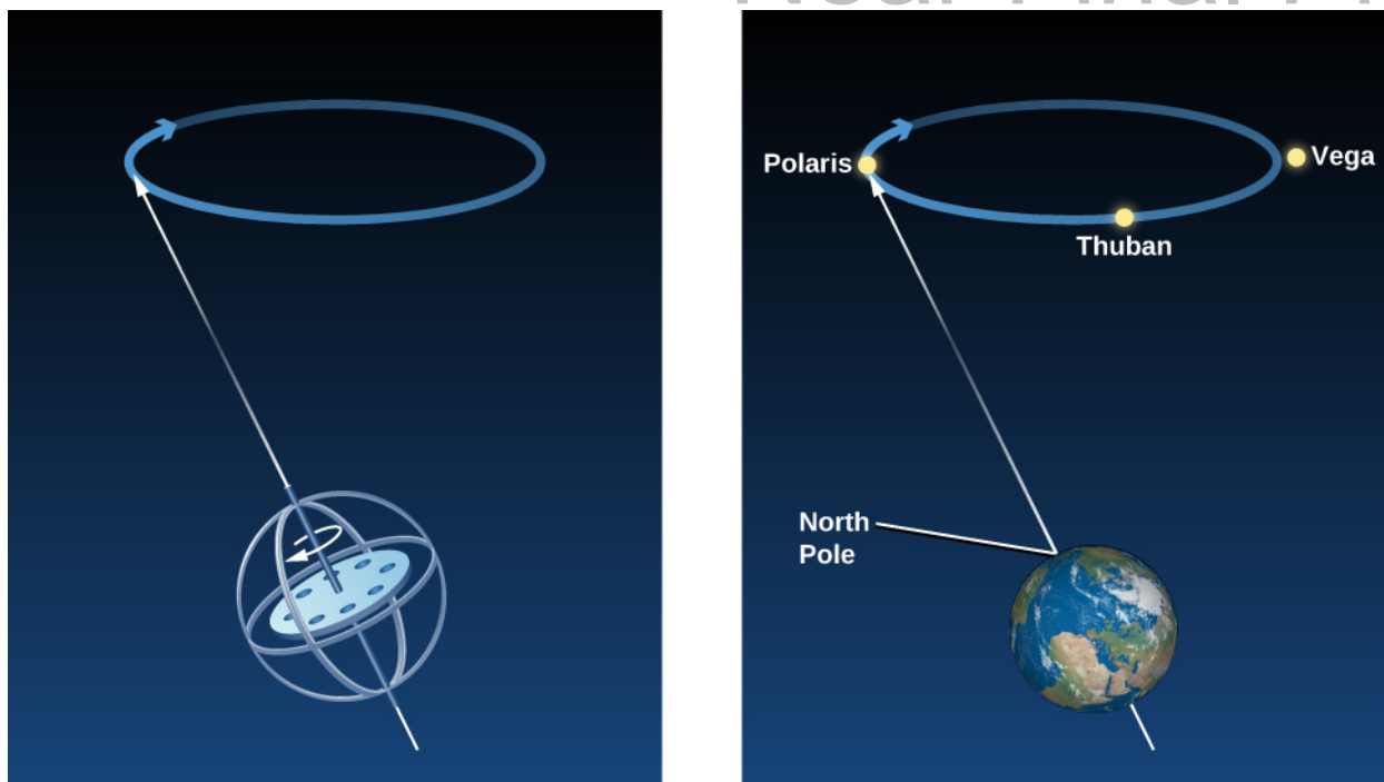
Figure 2.12. Precession. Just as the axis of a rapidly spinning top wobbles slowly in a circle, so the axis of Earth wobbles in a 26,000-year cycle. Today the north celestial pole is near the star Polaris, but about 5000 years ago it was close to a star called Thuban, and in 14,000 years it will be closest to the star Vega.
