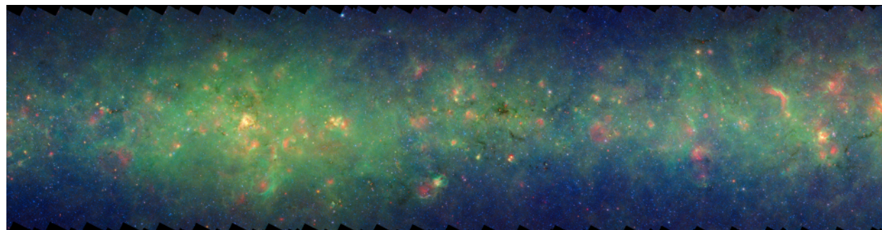
Figure 20.12. Infrared Emission from the Plane of the Milky Way. This infrared image taken by the Spitzer Space Telescope shows a field in the plane of the Milky Way. (Our Galaxy is in the shape of a frisbee; the plane of the Milky Way is the flat disk of that frisbee. Since the Sun, Earth, and solar system are located in the plane of the Milky Way and at a large distance from its center, we view the Galaxy edge on, much as we might look at a glass plate from its edge.) This emission is produced by tiny dust grains, which emit at 3.6 microns (blue in this image), 8.0 microns (green), and 24 microns (red). The densest regions of dust are so cold and opaque that they appear as dark clouds even at these infrared wavelengths. The red bubbles visible throughout indicate regions where the dust has been warmed up by young stars. This heating increases the emission at 24 microns, leading to the redder color in this image. (credit: modification of work by NASA/JPL-Caltech/University of Wisconsin)
