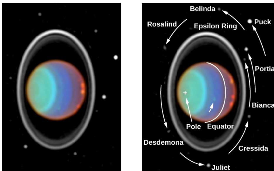
Figure 11.5. Infrared Image of Uranus. The infrared camera on the Hubble Space Telescope took these false-color images of the planet Uranus, its ring system, and satellites in 1997. The south pole of the planet (marked with a “+” on the right image) faces the Sun; its green color shows a strong local haze. The two images were taken 90 minutes apart, and during that time the five reddish clouds can be seen to rotate around the parallel to the equator. The rings (which are very faint in the visible light, but prominent in infrared) and eight satellites can be seen around the equator. This was the “bull’s eye” arrangement that Voyager saw as it approached Uranus in 1986. (credit: modification of work by Erich Karkoschka (University of Arizona), and NASA/ESA)
