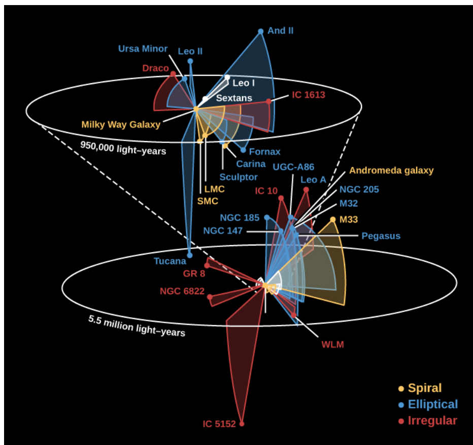
Figure 28.14. The Local Group. This illustration shows some members of the Local Group of galaxies, with our Milky Way at the center. The exploded view at the top shows the region closest to the Milky Way and fits into the bigger view at the bottom as shown by the dashed lines. The three largest galaxies among the three dozen or so members of the Local Group are all spirals; the others are small irregular galaxies and dwarf ellipticals. A number of new members of the group have been found since this map was made.
