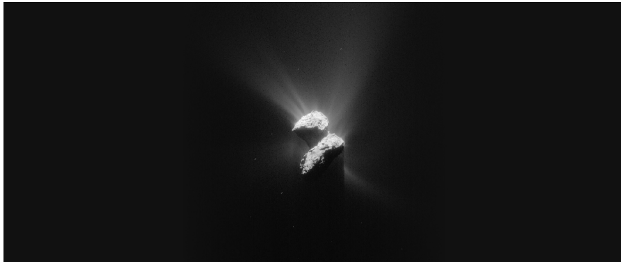
Figure 7.9. Comet Churyumov-Gerasimenko (67P). This image shows 67P near its closest approach to the Sun in 2015, as seen from the Rosetta spacecraft. Note the jets of gas escaping from the solid surface. (credit: ESA/Rosetta/NAVCAM, CC BY-SA IGO 3.0 ( http://creativecommons.org/licenses/by-sa/3.0/igo/ ))
