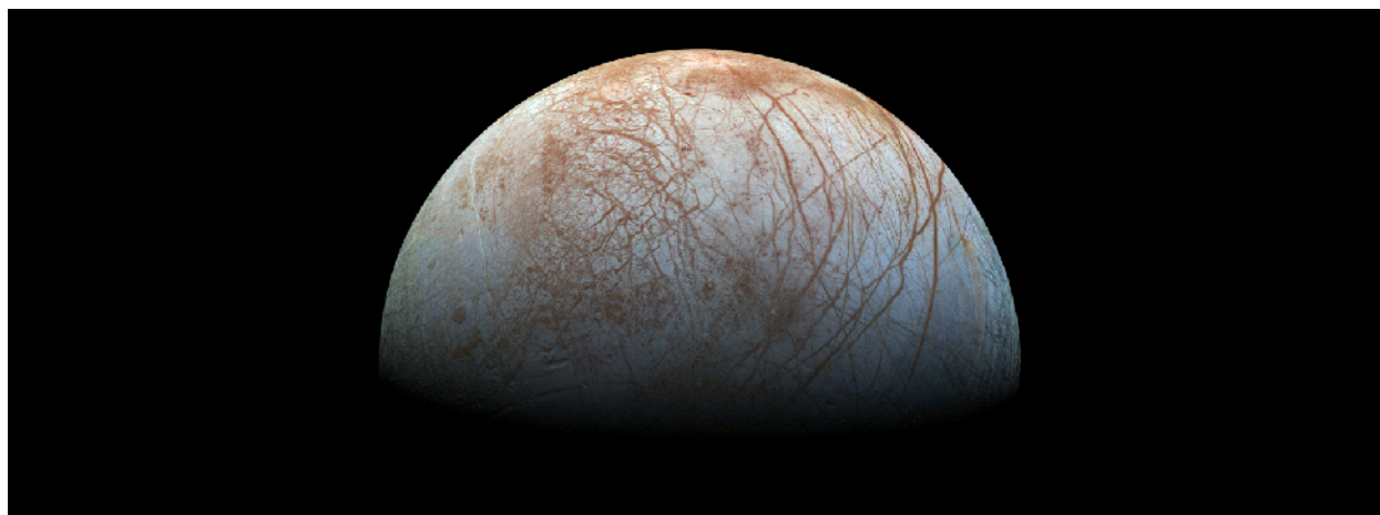
Figure 30.13. Jupiter's Moon Europa, as Imaged by NASA's Galileo Mission. The relative scarcity of craters suggests a surface that is "geologically young," and the network of colored ridges and cracks suggests constant activity and motion. Galileo's instruments also strongly suggested the presence of a massive ocean of salty liquid water beneath the icy crust. (credit: NASA/JPL-Caltech/SETI Institute)
