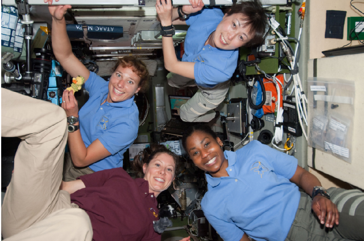
Figure 3.9. Astronauts in Free Fall. While in space, astronauts are falling freely, so they experience "weightlessness." Clockwise from top: Naoko Yamzaki (JAXA), Stephanie Wilson (NASA), Tracy Caldwell Dyson (NASA), and Dorothy Metcalf-Lindenburger (NASA). (credit: NASA)
