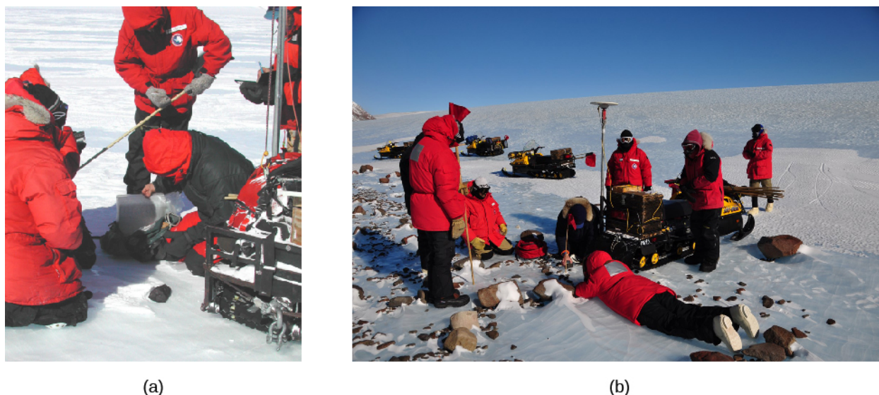
Figure 14.7. Antarctic Meteorite. (a) The US Antarctic Search for Meteorites (ANSMET) team recovers a meteorite from the Antarctic ice during a 2001–2002 mission. (b) The team is shown with some of the equipment used in the search. (credit a, b: modification of work by NASA)
