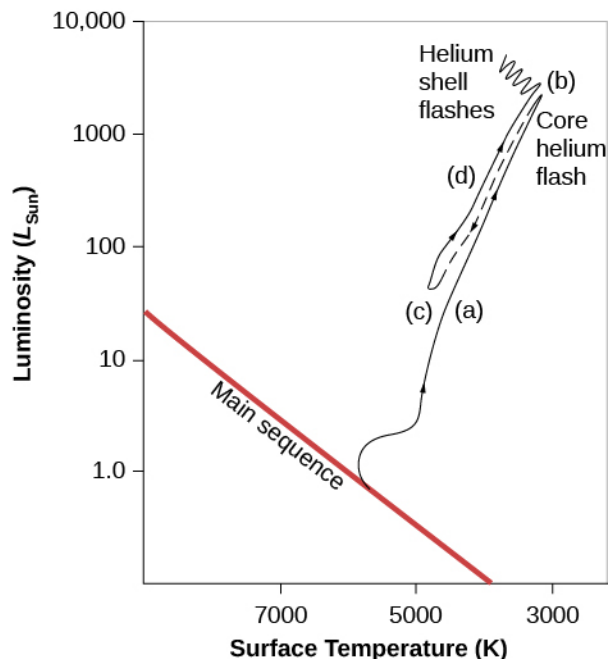
Figure 22.14. Evolution of a Star Like the Sun on an H-R Diagram. Each stage in the star's life is labeled. (a) The star evolves from the main sequence to be a red giant, decreasing in surface temperature and increasing in luminosity. (b) A helium flash occurs, leading to a readjustment of the star's internal structure and to (c) a brief period of stability during which helium is fused to carbon and oxygen in the core (in the process the star becomes hotter and less luminous than it was as a red giant). (d) After the central helium is exhausted, the star becomes a giant again and moves to higher luminosity and lower temperature. By this time, however, the star has exhausted its inner resources and will soon begin to die. Where the evolutionary track becomes a dashed line, the changes are so rapid that they are difficult to model.
