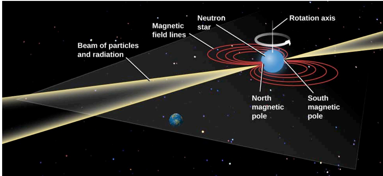
Figure 1. How a Pulsar Beam Sweeps Over the Earth
