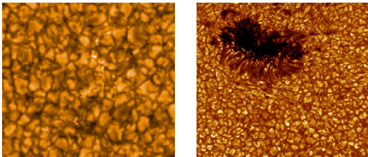
Figure 15.6. Granulation Pattern. The surface markings of the convection cells create a granulation pattern on this dramatic image taken from the Japanese Hinode spacecraft. You can see the same pattern when you heat up miso soup. (credit left: modification of work by Hinode JAXA/NASA/PPARC; credit right: ISP/SST/Oddbjorn Engvold, Jun Elin Wiik, Luc Rouppe van der Voort)
