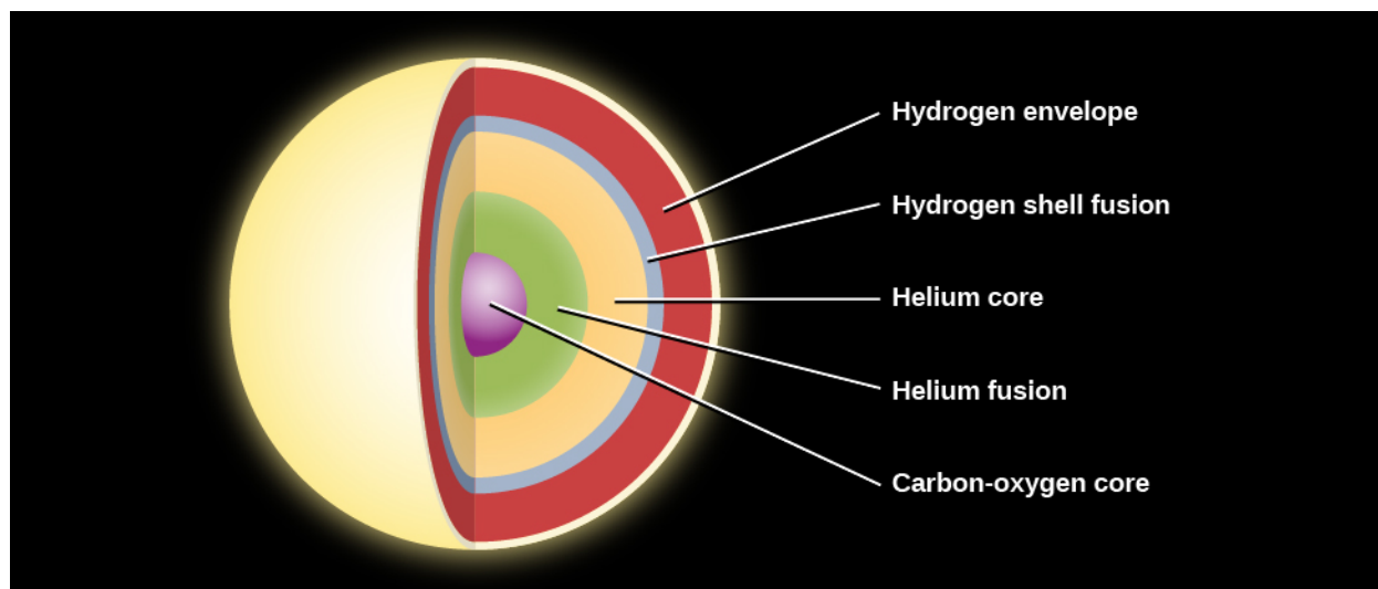
Figure 22.15. Layers inside a Low-mass Star before Death. Here we see the layers inside a star with a mass that is less than twice the mass of the Sun. These include, from the center outward, the carbon-oxygen core, a layer of helium hot enough to fuse, a layer of cooler helium, a layer of hydrogen hot enough to fuse, and then cooler hydrogen beyond.
