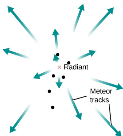
Figure 14.3. Radiant of a Meteor Shower. The tracks of the meteors diverge from a point in the distance, just as long, parallel railroad tracks appear to do. (credit “tracks”: Nathan Vaughn)
