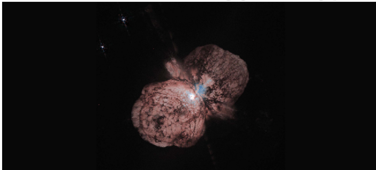
Figure 22.2. Eta Carinae. With a mass at least 100 times that of the Sun, the hot supergiant Eta Carinae is one of the most massive stars known. This Hubble Space Telescope image records the two giant lobes and equatorial disk of material it has ejected in the course of its evolution. The pink outer region is material ejected in an outburst seen in 1843, the largest of such mass loss event that any star is known to have survived. Moving away from the star at a speed of about 1000 km/s, the material is rich in nitrogen and other elements formed in the interior of the star. The inner blue-white region is the material ejected at lower speeds and is thus still closer to the star. It appears blue-white because it contains dust and reflects the light of Eta Carinae, whose luminosity is 4 million times that of our Sun. (credit: Jon Morse (University of Colorado) & NASA)
