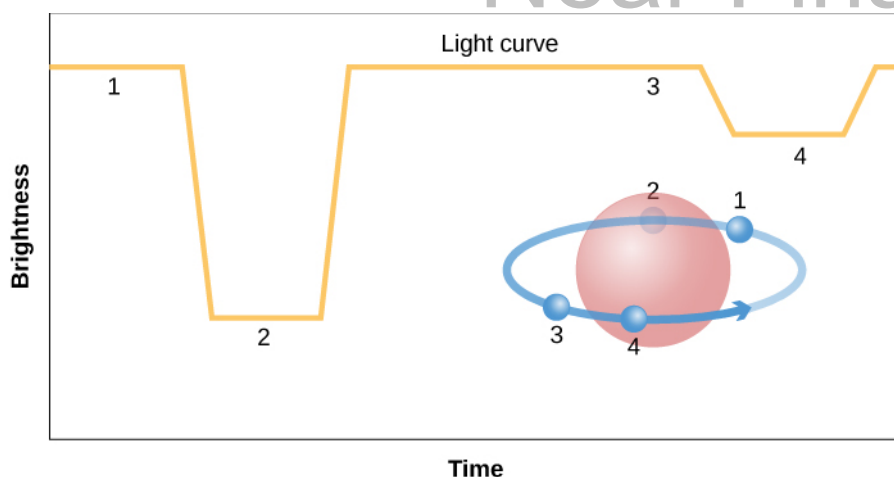
Figure 18.10. Light Curve of an Eclipping Binary. The light curve of an eclipsing binary star system shows how the combined light from both stars changes due to eclipses over the time span of an orbit. This light curve shows the behavior of a hypothetical eclipsing binary star with total eclipses (one star passes directly in front of and behind the other). The numbers indicate parts of the light curve corresponding to various positions of the smaller star in its orbit. In this diagram, we have assumed that the smaller star is also the hotter one so that it emits more flux (energy per second per square meter) than the larger one. When the smaller, hotter star goes behind the larger one, its light is completely blocked, and so there is a strong dip in the light curve. When the smaller star goes in front of the bigger one, a small amount of light from the bigger star is blocked, so there is a smaller dip in the light curve.
