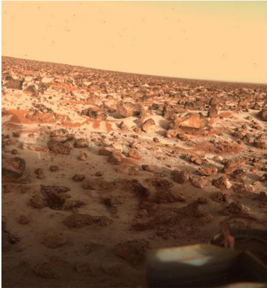
Figure 10.22. Water Frost in Utopia. This image of surface frost was photographed at the Viking 2 landing site during late winter. (credit: NASA/JPL)
