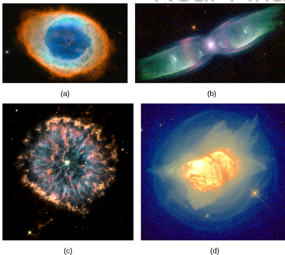
Figure 22.16. Gallery of Planetary Nebulae. This series of beautiful images depicting some intriguing planetary nebulae highlights the capabilities of the Hubble Space Telescope. (a) Perhaps the best known planetary nebula is the Ring Nebula (M57), located about 2000 light-years away in the constellation of Lyra. The ring is about 1 light-year in diameter, and the central star has a temperature of about 120,000 °C. Careful study of this image has shown scientists that, instead of looking at a spherical shell around this dying star, we may be looking down the barrel of a tube or cone. The blue region shows emission from very hot helium, which is located very close to the star; the red region isolates emission from ionized nitrogen, which is radiated by the coolest gas farthest from the star; and the green region represents oxygen emission, which is produced at intermediate temperatures and is at an intermediate distance from the star. (b) This planetary nebula, M2-9, is an example of a butterfly nebula. The central star (which is part of a binary system) has ejected mass preferentially in two opposite directions. In other images, a disk, perpendicular to the two long streams of gas, can be seen around the two stars in the middle. The stellar outburst that resulted in the expulsion of matter occurred about 1200 years ago. Neutral oxygen is shown in red, once-ionized nitrogen in green, and twice-ionized oxygen in blue. The planetary nebula is about 2100 light-years away in the constellation of Ophiuchus. (c) In this image of the planetary nebula NGC 6751, the blue regions mark the hottest gas, which forms a ring around the central star. The orange and red regions show the locations of cooler gas. The origin of these cool streamers is not known, but their shapes indicate that they are affected by radiation and stellar winds from the hot star at the center. The temperature of the star is about 140,000 °C. The diameter of the nebula is about 600 times larger than the diameter of our solar system. The nebula is about 6500 light-years away in the constellation of Aquila. (d) This image of the planetary nebula NGC 7027 shows several stages of mass loss. The faint blue concentric shells surrounding the central region identify the mass that was shed slowly from the surface of the star when it became a red giant. Somewhat later, the remaining outer layers were ejected but not in a spherically symmetric way. The dense clouds formed by this late ejection produce the bright inner regions. The hot central star can be seen faintly near the center of the nebulosity. NGC 7027 is about 3000 light-years away in the direction of the constellation of Cygnus. (credit a: modification of work by NASA, ESA, and the Hubble Heritage (STScI/AURA)-ESA/Hubble Collaboration; credit b: modification of work by Bruce Balick (University of Washington), Vincent Icke (Leiden University, The Netherlands), Garrelt Mellema (Stockholm University), and NASA; credit c: modification of work by NASA, The Hubble Heritage Team (STScI/AURA); credit d: modification of work by H. Bond (STScI) and NASA)
