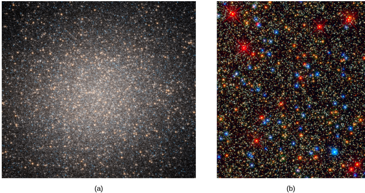
Figure 22.4. Omega Centauri. (a) Located at about 16,000 light-years away, Omega Centauri is the most massive globular cluster in our Galaxy. It contains several million stars. (b) This image, taken with the Hubble Space Telescope, zooms in near the center of Omega Centauri. The image is about 6.3 light-years wide. The most numerous stars in the image, which are yellow-white in color, are main-sequence stars similar to our Sun. The brightest stars are red giants that have begun to exhaust their hydrogen fuel and have expanded to about 100 times the diameter of our Sun. The blue stars have started helium fusion. (credit a: modification of work by NASA, ESA and the Hubble Heritage Team (STScI/AURA); credit b: modification of work by NASA, ESA, and the Hubble SM4 ERO Team)
