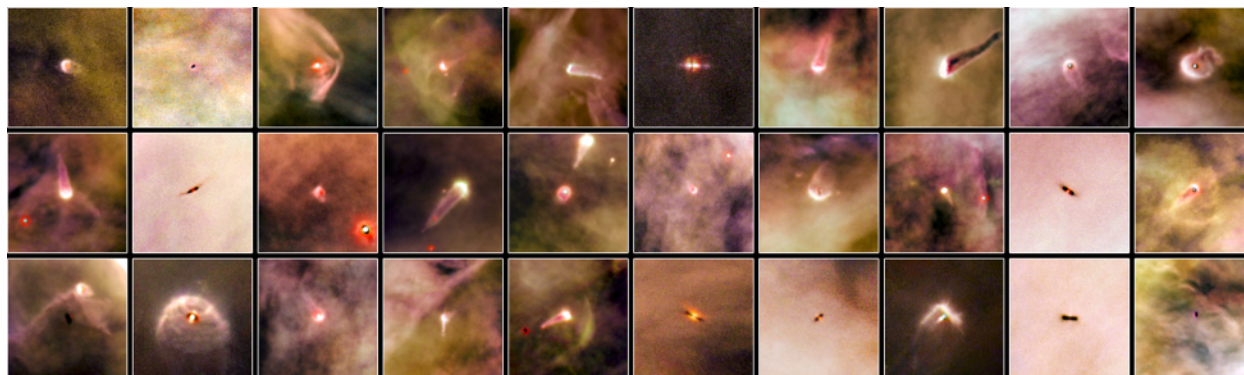
Figure 7.18. Atlas of Planetary Nurseries. These Hubble Space Telescope photos show sections of the Orion nebula, a relatively close-by region where stars are currently forming. Each image shows an embedded circumstellar disk orbiting a very young star. Seen from different angles, some are energized to glow by the light of a nearby star while others are dark and seen in silhouette against the bright glowing gas of the Orion nebula. Each is a contemporary analog of our own solar nebula—a location where planets are probably being formed today. (credit: modification of work by NASA/ESA, L. Ricci (ESO))
