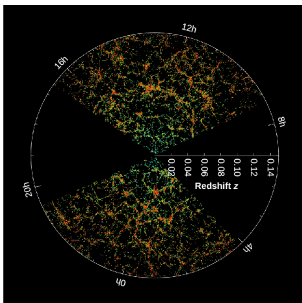
Figure 28.21. Sloan Digital Sky Survey Map of the Large-Scale Structure of the Universe. This image shows slices from the SDSS map. The point at the center corresponds to the Milky Way and might say “You Are Here!” Points on the map moving outward from the center are farther away. The distance to the galaxies is indicated by their redshifts (following Hubble’s law), shown on the horizontal line going right from the center. The redshift z = \Delta\lambda/\lambda , where \Delta\lambda is the difference between the observed wavelength and the wavelength \lambda emitted by a nonmoving source in the laboratory. Hour angle on the sky is shown around the circumference of the circular graph. The colors of the galaxies indicate the ages of their stars, with the redder color showing galaxies that are made of older stars. The outer circle is at a distance of two billion light-years from us. Note that red (older stars) galaxies are more strongly clustered than blue galaxies (young stars). The unmapped areas are where our view of the universe is obstructed by dust in our own Galaxy. (credit: M. Blanton and the Sloan Digital Sky Survey)
