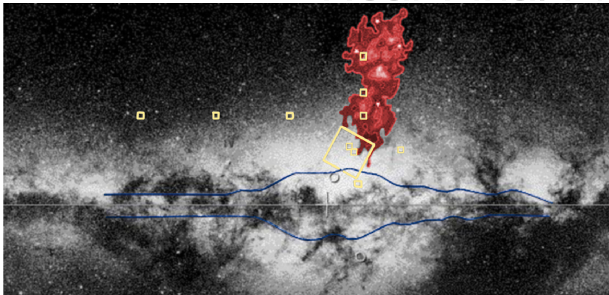
Figure 25.22. Sagittarius Dwarf. In 1994, British astronomers discovered a galaxy in the constellation of Sagittarius, located only about 50,000 light-years from the center of the Milky Way and falling into our Galaxy. This image covers a region approximately 70^\circ \times 50^\circ and combines a black-and-white view of the disk of our Galaxy with a red contour map showing the brightness of the dwarf galaxy. The dwarf galaxy lies on the other side of the galactic center from us. The white stars in the red region mark the locations of several globular clusters contained within the Sagittarius dwarf galaxy. The cross marks the galactic center. The horizontal line corresponds to the galactic plane. The blue outline on either side of the galactic plane corresponds to the infrared image in Figure 25.7 . The boxes mark regions where detailed studies of individual stars led to the discovery of this galaxy. (credit: modification of work by R. Ibata (UBC), R. Wyse (JHU), R. Sword (IoA))
