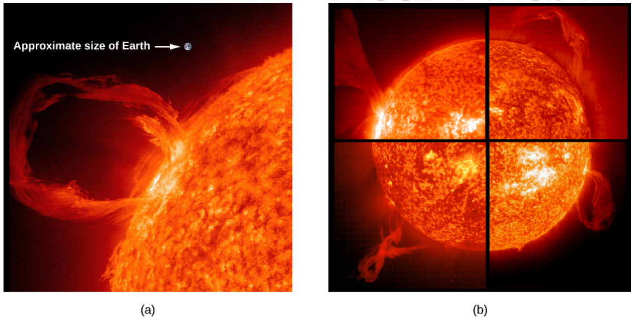
Figure 15.19. Prominences. (a) A prominence is a huge cloud of relatively cool (about 60,000 K in this case), fairly dense gas suspended in the much hotter corona. These pictures, taken in ultraviolet, are color coded so that white corresponds to the hottest temperatures and dark red to cooler ones. The four images were taken, moving clockwise from the upper left, on May 15, 2001; March 28, 2000; January 18, 2000; and February 2, 2001. (b) This image of an eruptive prominence was taken in the light of singly ionized helium in the extreme ultraviolet part of the spectrum. The prominence is a particularly large one. An image of Earth is shown at the same scale for comparison. (credit a: modification of work by NASA/SOHO; credit b: modification of work by NASA/SDO)
