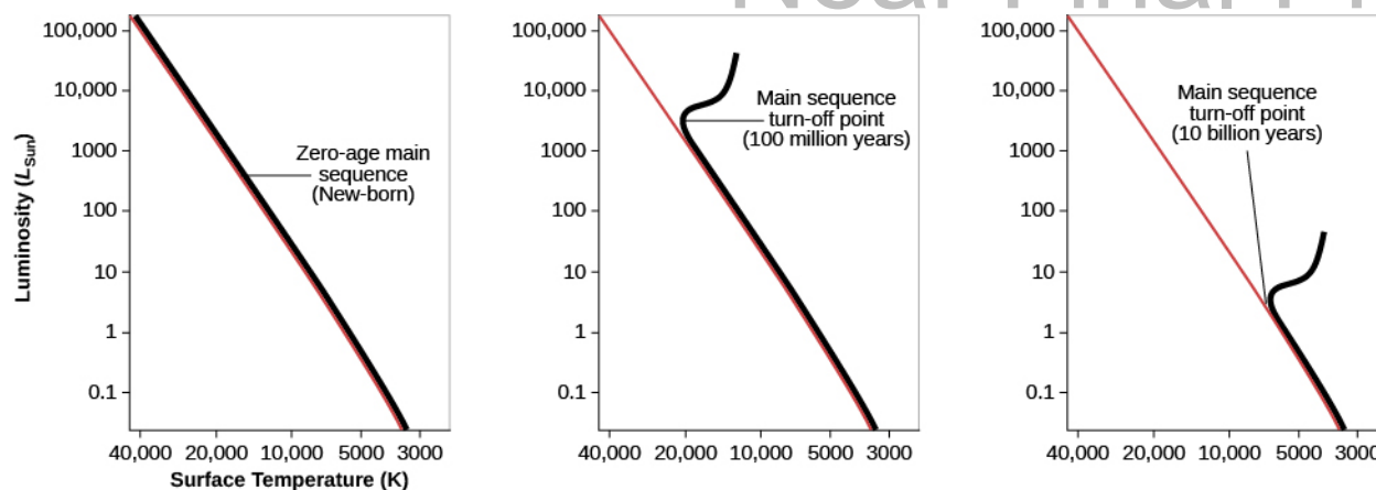
Figure 22.13. H-R Diagrams for Clusters of Different Ages. This sketch shows how the turn-off point from the main sequence gets lower as we make H-R diagrams for clusters that are older and older.
