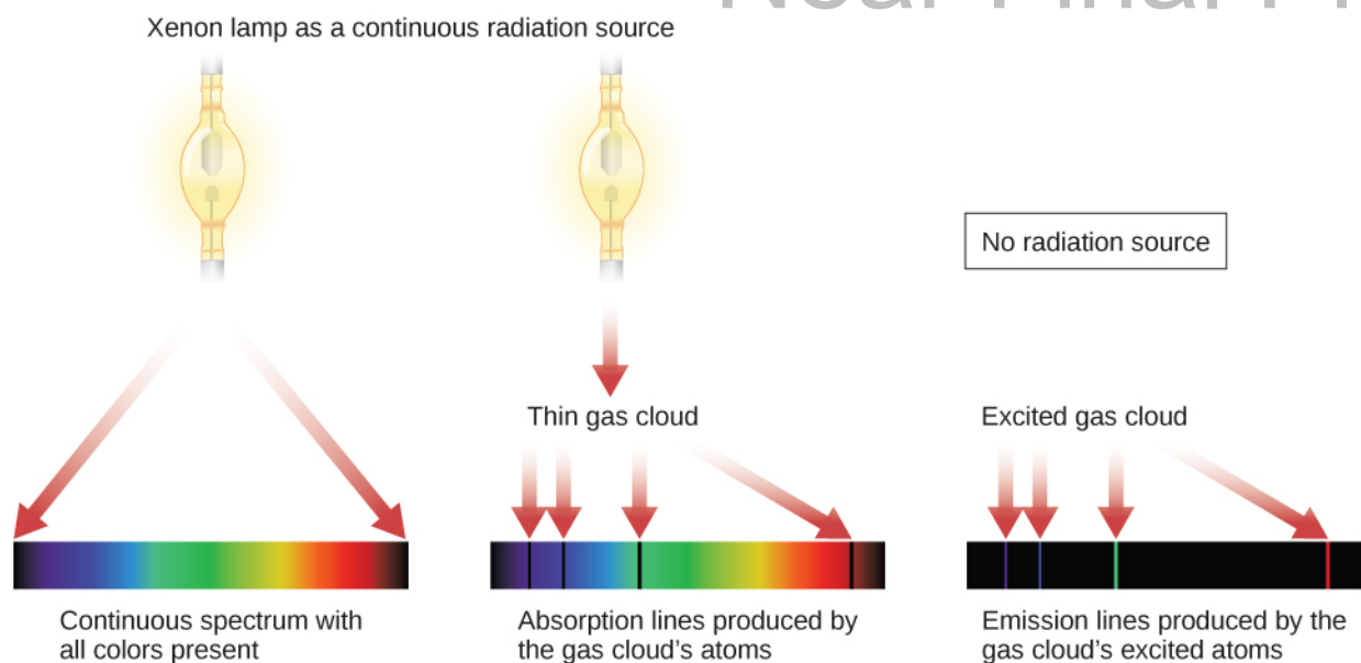
Figure 5.21. Three Kinds of Spectra. When we see a lightbulb or other source of continuous radiation, all the colors are present. When the continuous spectrum is seen through a thinner gas cloud, the cloud's atoms produce absorption lines in the continuous spectrum. When the excited cloud is seen without the continuous source behind it, its atoms produce emission lines. We can learn which types of atoms are in the gas cloud from the pattern of absorption or emission lines.
