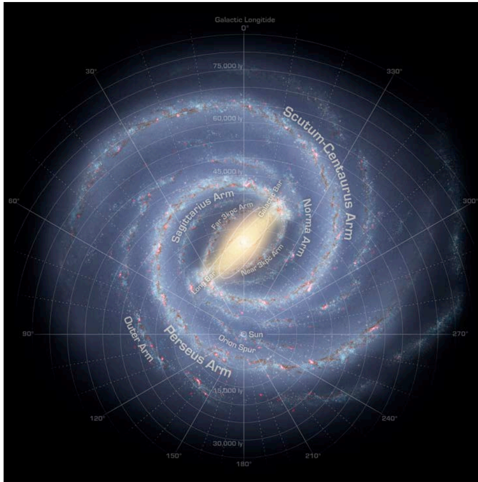
Figure 2. The Structure of the Milky Way Galaxy
