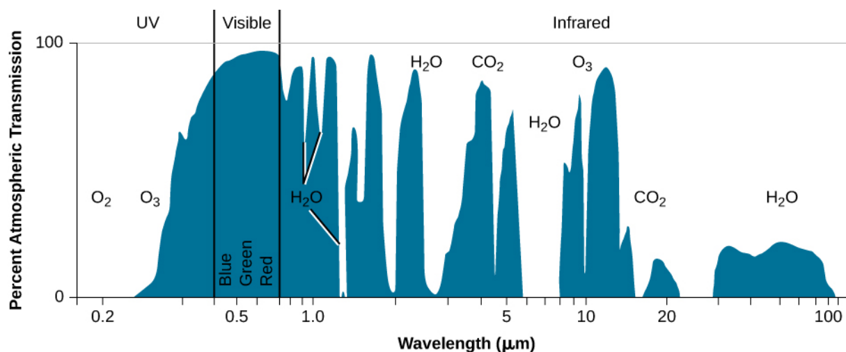
Figure 30.17. Spectrum of Light Transmitted through Earth’s Atmosphere. This graph shows wavelengths ranging from visible (far left) to infrared. The many downward “spikes” come from absorption of particular wavelengths by molecules in Earth’s atmosphere. Some of these compounds, like water and the combination oxygen/ozone and methane, might reveal Earth as both habitable and inhabited. We will have to rely on this sort of information to seek life on exoplanets, but our spectra will be of much poorer quality than this one, in part because we will receive so little light from the planet. (credit: modification of work by NASA)
