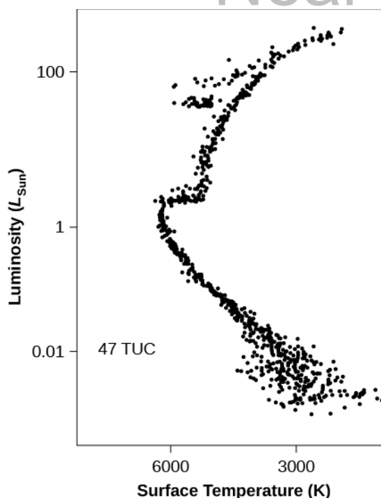
Figure 22.12. Cluster 47 Tucanae. This H-R diagram is for the globular cluster 47. Note that the scale of luminosity differs from that of the other H-R diagrams in this chapter. We are only focusing on the lower portion of the main sequence, the only part where stars still remain in this old cluster.
