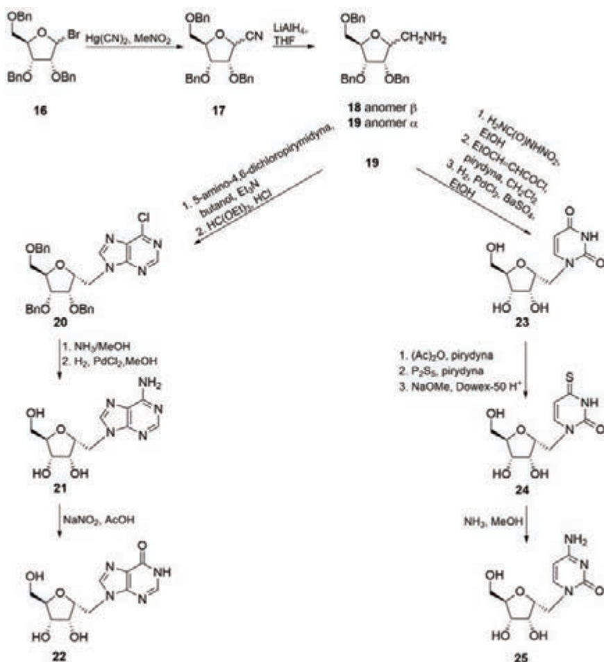
Schemat 4. Synteza \alpha 1'-homoadenozyny 21 , 1'-homioinozyny 22 , 1'-homourydyny 23 , 1'-homocytydyny 25 Scheme 4. Synthesis of \alpha 1'-homoadenine 21 , 1'-homioinosine 22 , 1'-homouridine 23 , 1'-homocytidine 25
