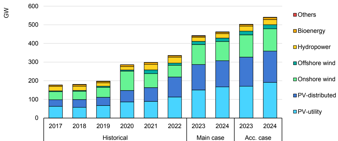
Net renewable electricity capacity additions by technology, historical, main and accelerated cases
