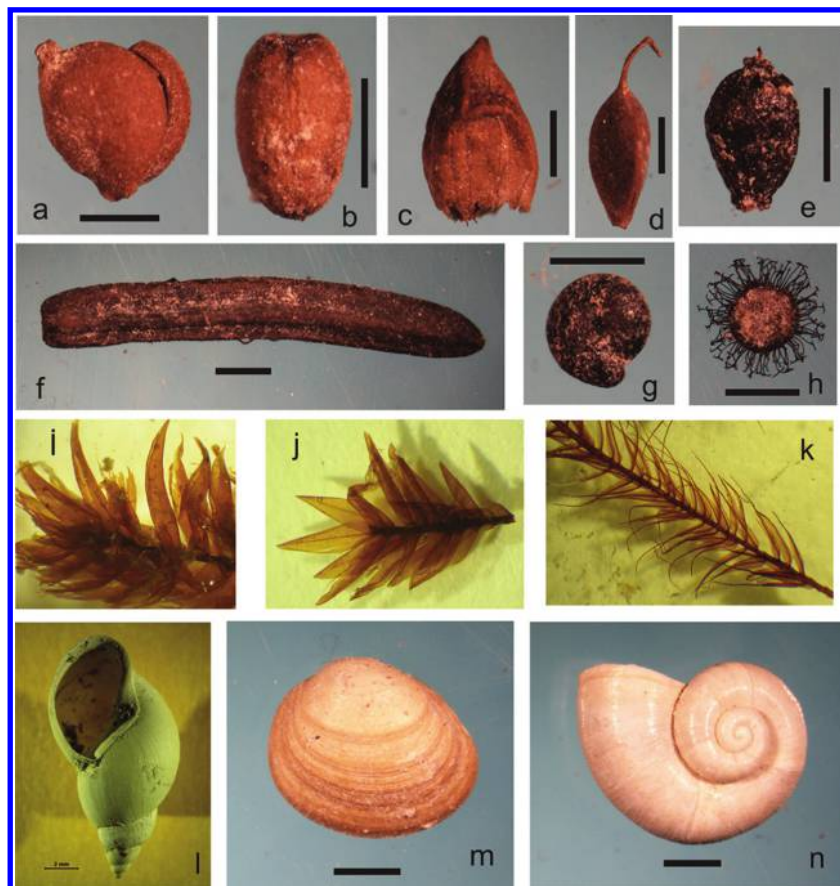
Fig. 7. Macrofossils recovered from sediment associated with the bison skeleton. (a) Potamogeton nutlet; (b) Hippuris seed; (c) Carex perigynia; (d) Carex achene; (e) Eleocharis achene; (f) Picea needle; (g) Chenopodium seed; (h) Cristatella mucedo statoblast; (i) Scorpidium scorpioides stem with leaves; (j) Calliergon giganteum stem with leaves; (k) Drepanocladus longifolius stem with leaves; (l) Stagnicola arctica shell; (m) Valvata sincera bivalve shell; (n) Pisidium casertanum shell.
