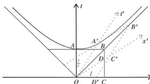
Fig. 2. Minkowski's spacetime diagram [6]
