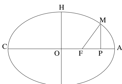
Fig. 1. Poincaré's light ellipse
