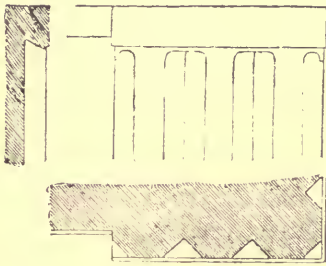
FIG. 20.—DETAILS OF THE TRIGLYPH.
