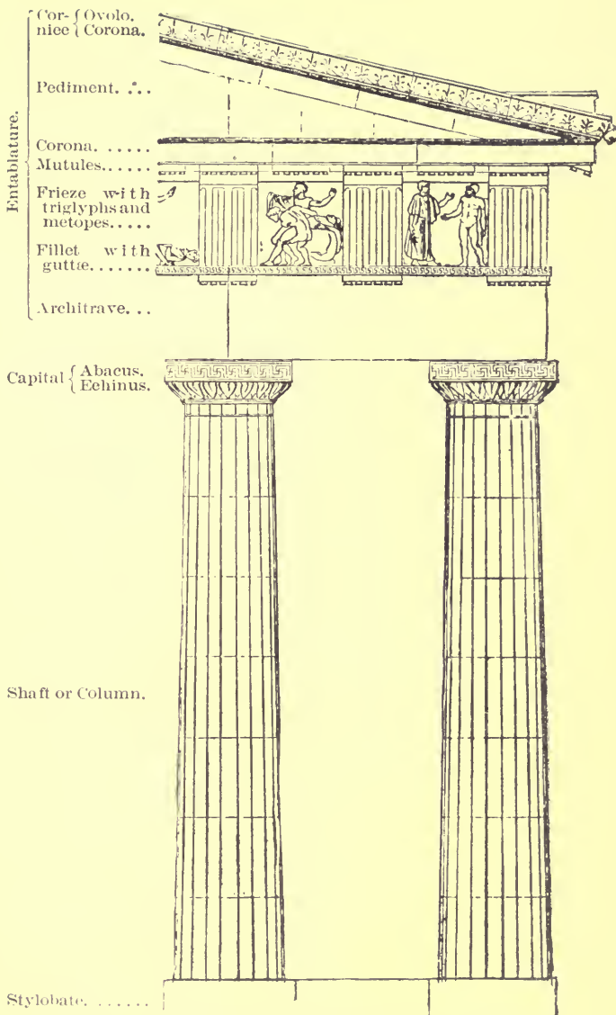
FIG. 11.—THE GREEK DORIC ORDER FROM THE THESEUM.
