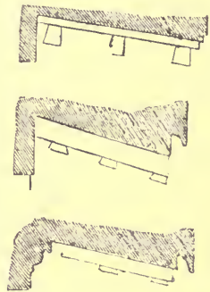
FIG. 21.—DETAILS OF THE MUTULES.
