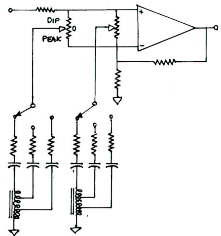
FIG 2A - FEEDBACK L-C EQUALIZER (Peak and Dip)
