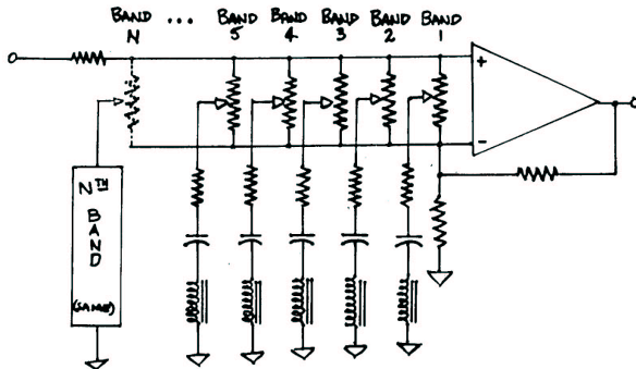
FIG 2B - FEEDBACK L-C GRAPHIC EQUALIZER (Multiple Peak)
