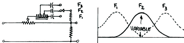
FIG 1E - VARIABLE FREQUENCY PEAK
