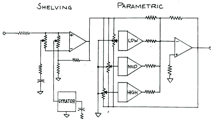
FIG 10 - FULL SYSTEM with three parametric peaks and two shelves
