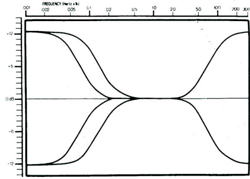
FIG 11 - SHELVING CURVES
