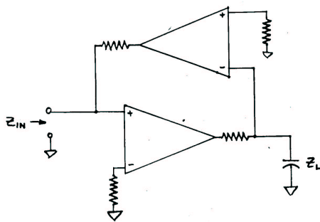
FIG 3 - SIMPLE GYRATOR
