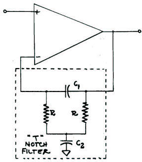
FIG 6 - PEAK INVERSION
