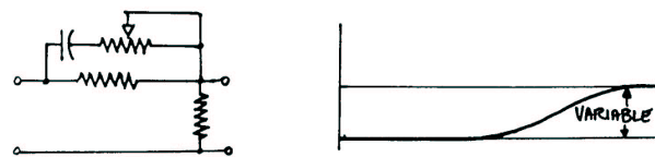
FIG 1C - VARIABLE HIGH FREQUENCY SHELF
