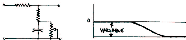
FIG 1A - VARIABLE LOW FREQUENCY SHELF
