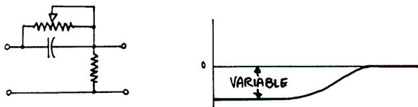
FIG 1B - VARIABLE LOW FREQUENCY DROOP
