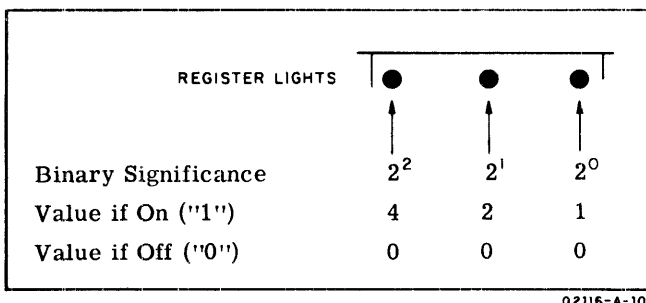
Figure 3-2. Composition of Octal Digit
