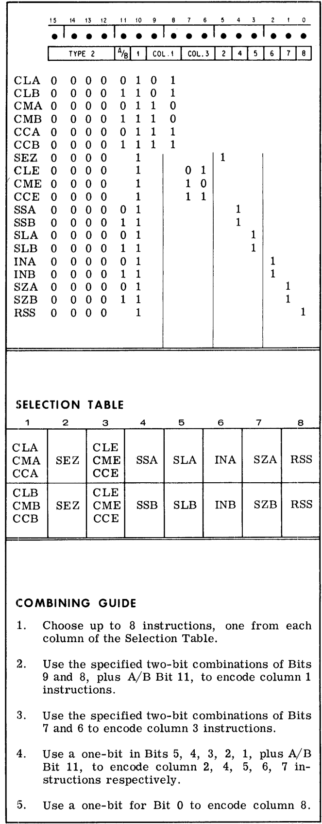
Figure 2-6. Alter-Skip Instructions
