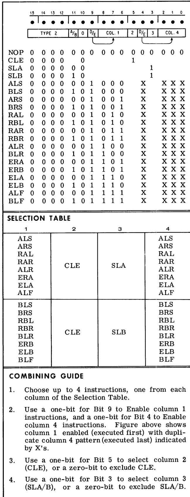
Figure 2-5. Shift-Rotate Instructions
