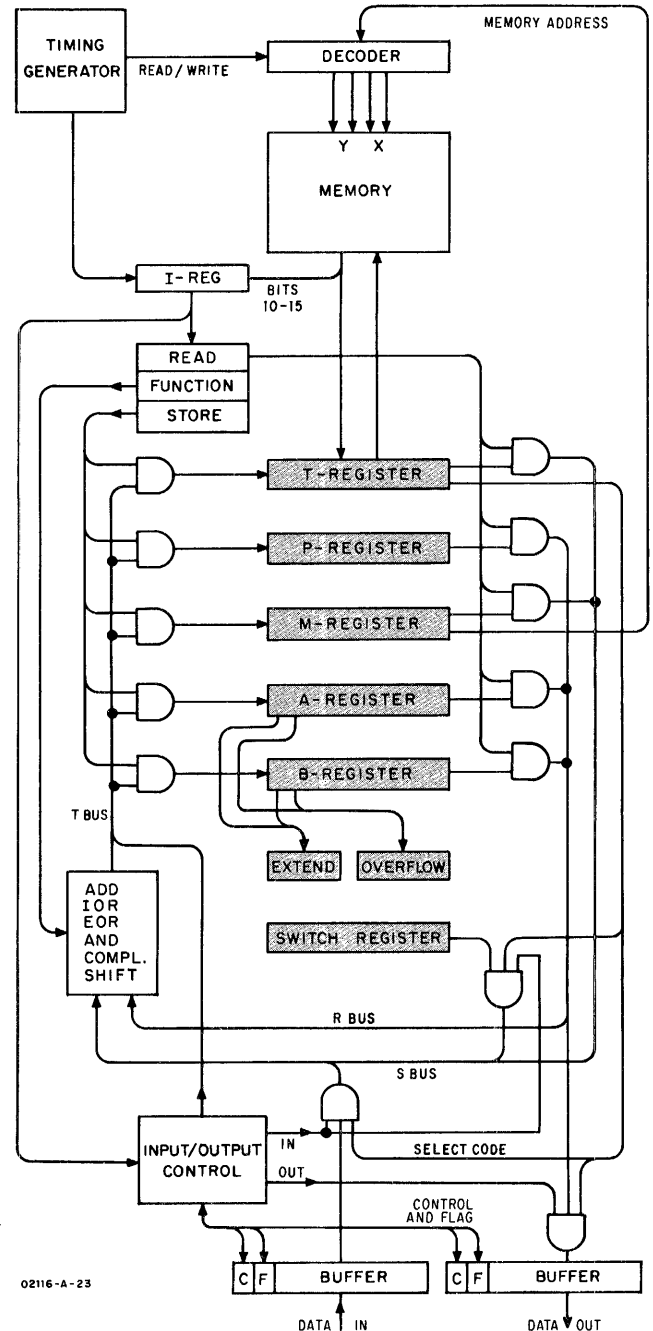
Figure 3-1. HP 2116A Simplified Block Diagram
