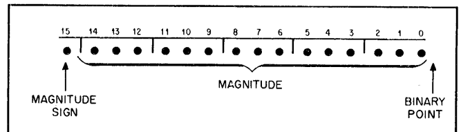
Figure 2-8. Basic Data Format
