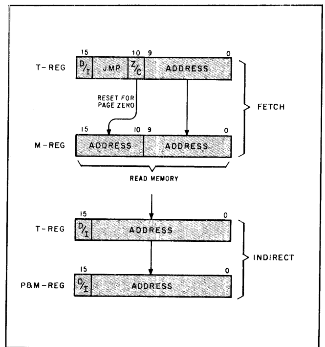
Figure 3-18. Register Manipulations for Indirect Jump
