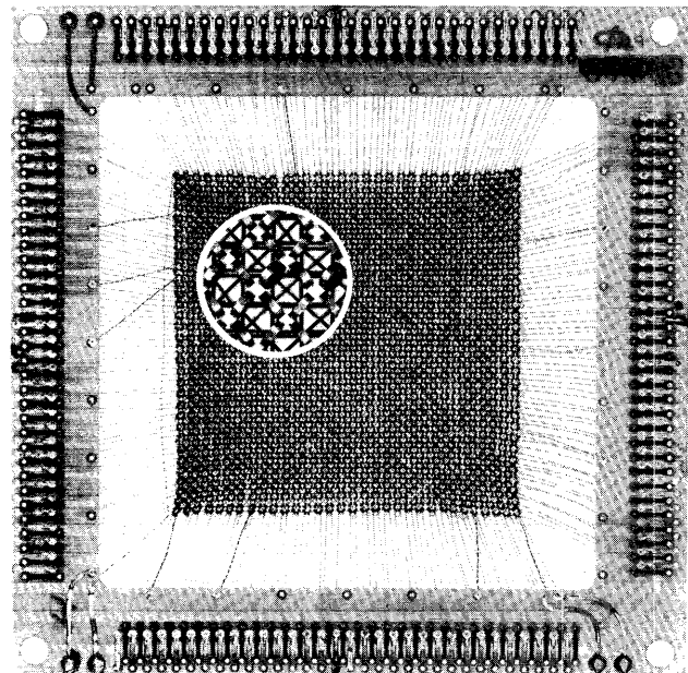
Figure 3-10. Core Plane
