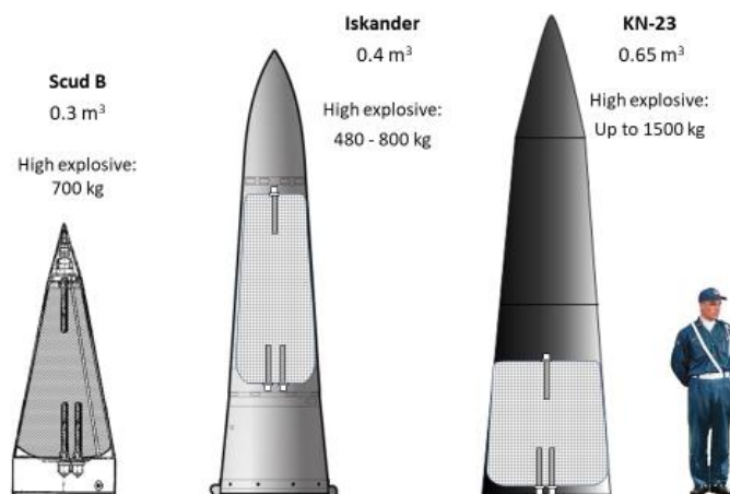
Figure 21. Volume and mass of the military payload of the SS-1c/Scud B, the SS-26 E or M, and estimation of the maximum mass of that of the KN-23 and KN23A
