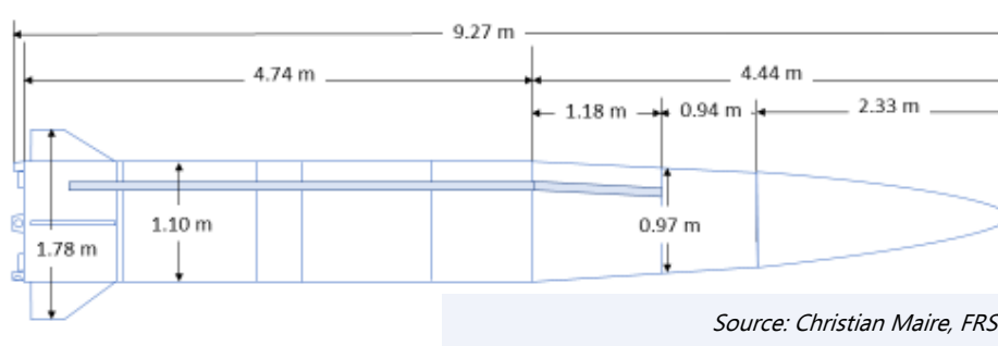
Figure 31. KN-23 and KN-23A upper sections
