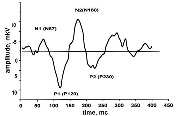
Figure 2. Example of visual evoked potential of differences (EPD) in response to abrupt stimulus change. The most defined components of this potential are two positive and two negative peaks. Our previous studies (Izmailov et al, 1998, 2004) showed that: (a) The amplitude of the N1 component monotonously increases not only with an increase in the chromatic difference between stimuli, but also with increase in achromatic difference; (b) Peak N1 amplitude correlates with the N1P1 inter-peak amplitude; (c) The latent period of this component varies between the 50-100ms range. The amplitudes of the following EPD components are monotonously linked with configuration differences between stimuli, represented by separate lines (Paramey, 1996) or by a combination of several lines (linear pattern) (Izmailov et al., 1999). The P1 amplitude correlates with the P1N2 inter-peak amplitude, and the N2 amplitude correlates with the N2P2 inter-peak amplitude. Therefore in our studies, we usually analyze amplitude and latency stability.
