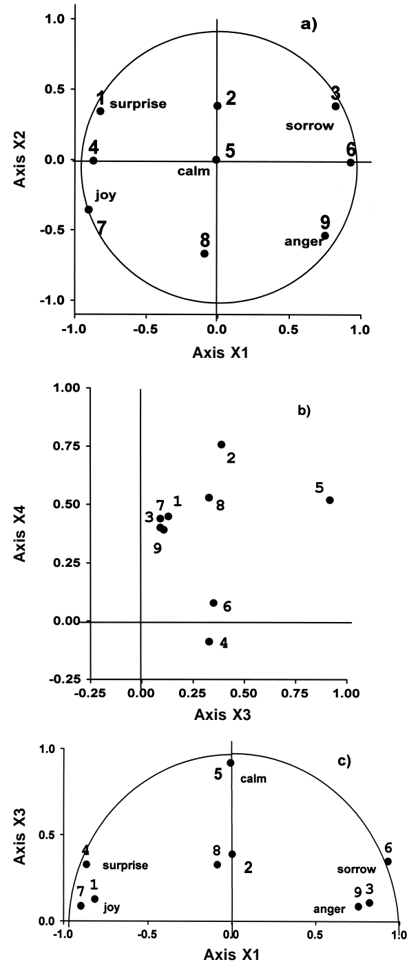
Figure 3. Projection of 9 schematic face-points on three planes: (a) X1X2, (b) X3X4, and (c) X1X3 of a four-dimension space derived through multidimensional scaling of dissimilarities estimates. Point numbers correspond to faces numbers of Figure 1. The emotional characteristics of some of the faces are derived from previous studies (Izmailov et al, 1999) (commentary in the text). On the graph, the noise zone corresponding to 10% error is represented by a circle around the stimulus-point.
